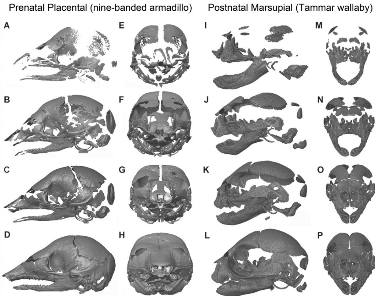
Fig. 1 Comparative skull ossification for four prenatal stages of placental, Dasyus novemcinctus , the nine-banded armadillo (A–H), and four postnatal stages of a marsupial, Macropus eugenii , the Tammar wallaby (I–P), demonstrating the clear differences level of cranial ossification of birth. All of the prenatal armadillo stages (A–H) show greater ossification of the skull than the earliest postnatal stage of the wallaby (I, M), and the latest sampled prenatal armadillo (D, H) is more ossified than a 6–8 week old wallaby (L, P; wallaby age estimate from Ramirez-Chaves et al. 2016). (A)–(D) and (I)–(L) are lateral views, and (E)–(H) and (M)–(P) are anterior views, proceeding from earliest to latest stages sampled from top to bottom. Dasyus novemcinctus specimens are: (A) and (E), 85893b; (B) and (F), 12XII01a; (C) and (G), A5022; (D) and (H), 40647. Macropus eugenii specimens are: (I) and (M), Meug1621; (J) and (N), Meug1694; (K) and (O), Meug1682_Yellow; and (L) and (P), Meug1716_yellow.
