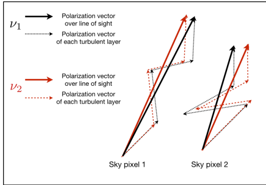
Fig. 7. Schematic illustration of the decomposition of the line of sight polarization pseudo-vector into a random walk process through four turbulent layers, shown for two neighbouring pixels at two frequencies, \nu_1 and \nu_2 . The integrated polarization pseudo-vectors are affected by the polarization angle fluctuations, leading to a decorrelation between the two frequencies.
