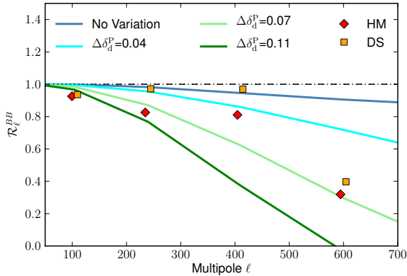
Fig. 5. Correlation ratio modelled with Gaussian spatial variations of the polarized dust spectral index, in LR42 as in Fig. 2. The HM and DS Planck measurements are shown as diamonds and squares, respectively. The model is plotted for four values of \Delta\delta_d^p , which is defined as the standard deviation of the Gaussian realization of the spectral index after smoothing at 1^\circ . The first model, with \Delta\delta_d^p = 0 , is described in Sect. 3.2.
