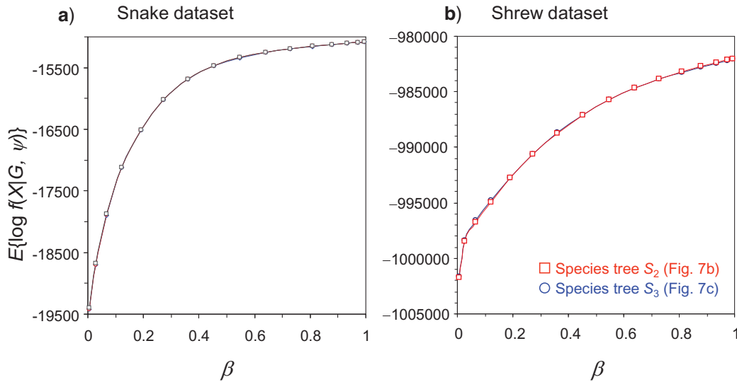
FIGURE 7. Calculation of the marginal likelihood for fixed species trees. The average log likelihood over the MCMC sample from the posterior is plotted against the given \beta for each fixed species tree. In a) the 3 alternative species trees for the rattlesnake dataset are compared: MB-S (which is the MAP tree), MS-B, and BS-M (Fig. 6). The three curves are indistinguishable. In b), the 2 curves are for the species trees S_2 and S_3 of Philippine shrews for the UCE dataset (Fig. 8).
