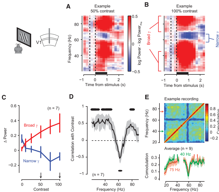
Figure 2. Narrowband Gamma Oscillations Are Suppressed by Visual Contrast (A and B) LFP spectrogram averaged over 20 presentations of a drifting grating stimulus at 50% contrast (A) and 100% contrast (B) in a single experiment. Color shows power relative to pre-stimulus baseline (−0.5 to 0 s); bars below indicate the period of presentation of a 50° sinusoidal drifting grating in the retinotopic location of the recorded area. (C) Power at the end of the stimulus presentation period (1 s) as a function of visual contrast for narrowband gamma (blue, calculated as the mean across the 55–65 Hz band) and broadband gamma (red, calculated as the mean across bands 20–40 and 70–90 Hz). The small increase in narrowband gamma power for zero contrast (blank) stimuli likely reflects continuing recovery from suppression by the preceding stimulus. Error bars show mean \pm SEM. (D) Correlation of power at different frequencies with contrast. Shaded area shows the mean \pm SEM across experiments ( n = 7 ); dots above/below the curve indicate frequencies with significant positive/negative correlations ( p < 0.05 ; n = 7 ). (E) Comodulation of power at different frequencies, i.e., the correlation in the power of different frequency bands, in an example recording. The blue cross visible at 60 Hz indicates that narrowband gamma power is uncorrelated with broadband gamma power. Bottom: comodulation of two frequencies of broadband gamma, 40 Hz (green) and 75 Hz (red), with respect to other frequency bands, showing a dip at narrowband gamma frequency. Shaded area shows the mean \pm SEM across nine recordings in a virtual reality environment. Arrows indicate the frequencies shown in the bottom plots.
