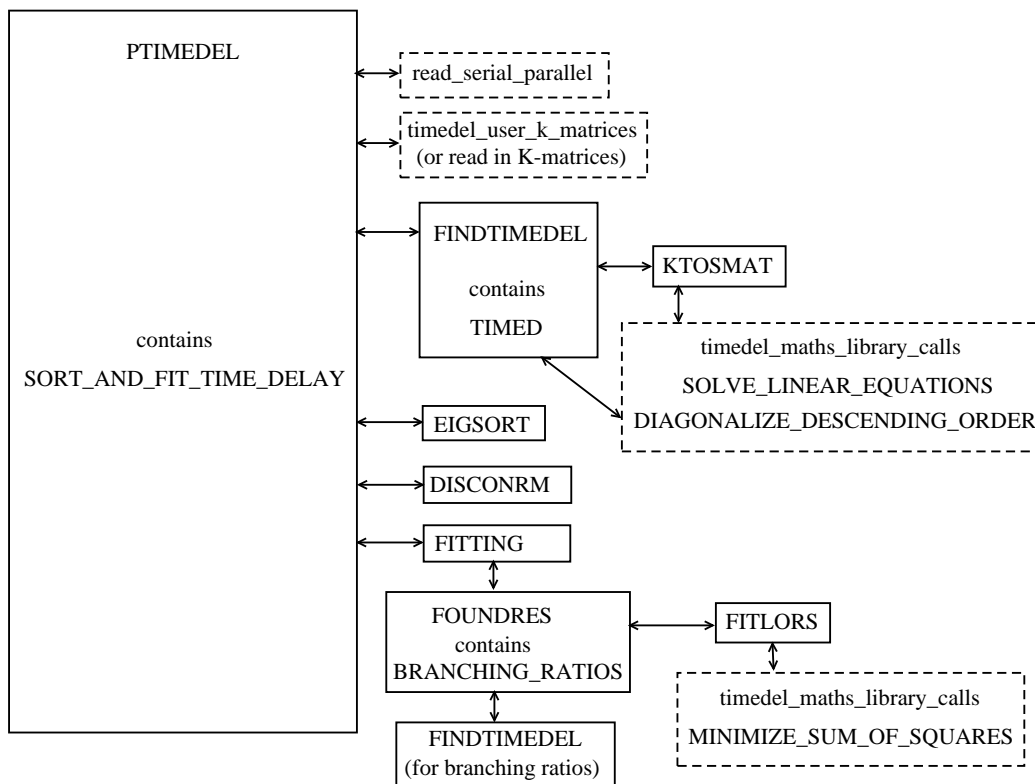
Figure 3: The ‘physics code’ call structure for routine PTIMEDEL. Dashed line boxes represent routines outside module timedel_module. The calls to module serial_parallel are omitted for space and clarity, and are described in the text.
