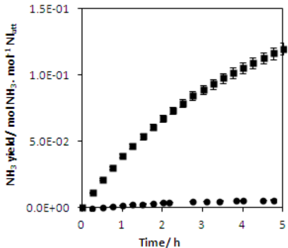
Figure 10. Ammonia yield of A-Mn-N with 60 \text{ ml min}^{-1} of 1:3 \text{ N}_2: \text{H}_2 at 400^\circ\text{C} : (●) K-Mn-N, (■) Li-Mn-N. Error propagation within a 95% confidence interval.
