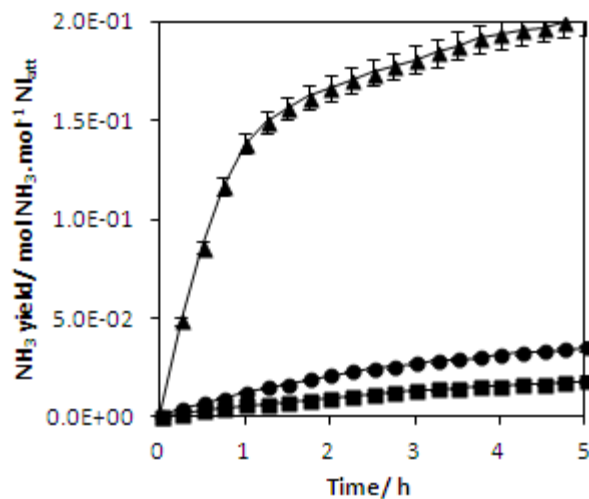
Figure 12. Regenerability of Li-Mn-N: (▲) first cycle, (●) second cycle and (■) third cycle. Reduction step conducted with 60 \text{ ml min}^{-1} of 1:3 Ar: \text{H}_2 at 400^\circ\text{C} . The nitridation step was conducted with 60 \text{ ml min}^{-1} flow of \text{N}_2 at 800^\circ\text{C} . Error propagation within a 95% confidence interval.
