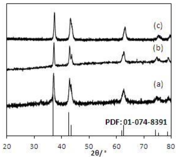
Figure 7. XRD patterns collected after the nitridation step. (a) \text{Mn}_3\text{N}_2 , (b) K-Mn-N, (c) Li-Mn-N.
