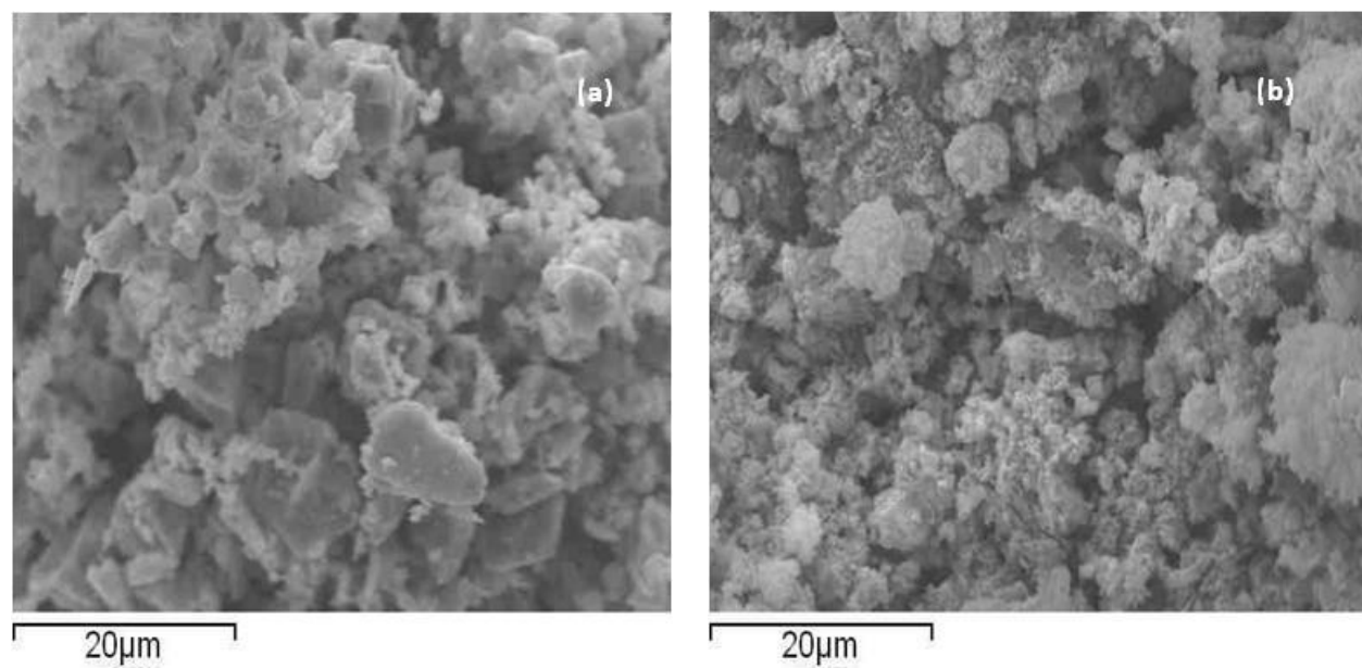
Figure 3. SEM micrographs of (a) \text{Mn}_2\text{O}_3 , (b) \text{Mn}_3\text{N}_2 .
