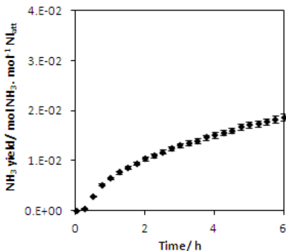
Figure 8. Ammonia yield of \text{Mn}_3\text{N}_2 with 60 \text{ ml min}^{-1} of 1:3 \text{ N}_2: \text{H}_2 at 400^\circ\text{C} . Error propagation within a 95% confidence interval.
