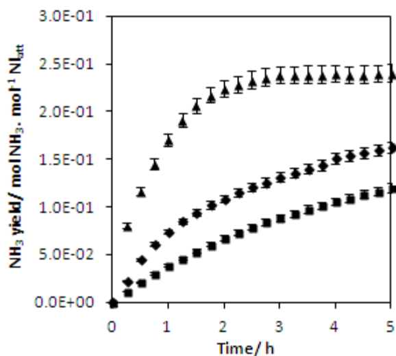
Figure 10. Ammonia yield of A-Mn-N with 60 \text{ ml min}^{-1} of 1:3 \text{ N}_2: \text{H}_2 at 400^\circ\text{C} : (●) K-Mn-N, (■) Li-Mn-N. Error propagation within a 95% confidence interval.
