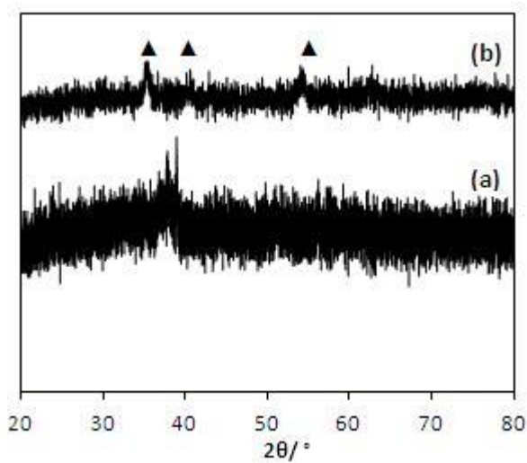
Figure 5. XRD patterns collected after the nitridation step of: (a) Co-Mn-O, (b) Mn-Fe-O.
