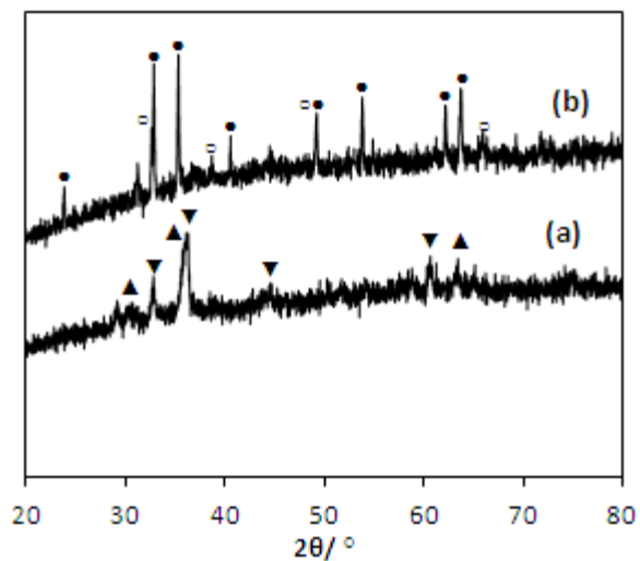
Figure 4. XRD patterns collected after calcination step of (a) Co-Mn-O: ▲ \text{CoMn}_2\text{O}_4 (PDF number: 00-055-068) ▼ \text{Co}_2\text{MnO}_4 (PDF number: 00-023-1237), (b) Mn-Fe-O: ● \text{Fe}_2\text{O}_3 (PDF number: 01-085-0987) ○ \text{Mn}_2\text{O}_3 (PDF number: 01-078-0390).
