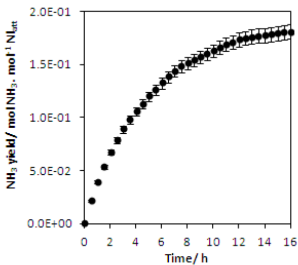
Figure 13. Ammonia yield of Li-Mn-N with 60 \text{ ml min}^{-1} of 1:3 \text{N}_2 : \text{H}_2 at 400^\circ\text{C} for 16h. Error propagation within a 95% confidence interval.
