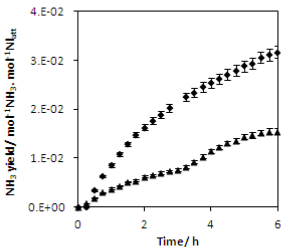
Figure 9. Ammonia yield of A-Mn-N with 60 \text{ ml min}^{-1} of 1:3 \text{ N}_2: \text{H}_2 at 400^\circ\text{C} : (▲) Fe-Mn-N, (◆) Co-Mn-N. Error propagation within a 95% confidence interval.
