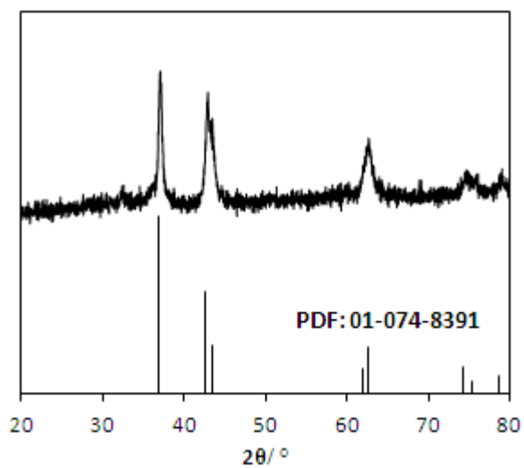
Figure 2. XRD patterns collected after the nitridation of \text{Mn}_2\text{O}_3 .
