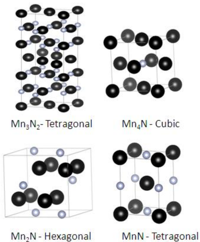
Figure 1. Manganese nitride structures adapted from reference [22].
