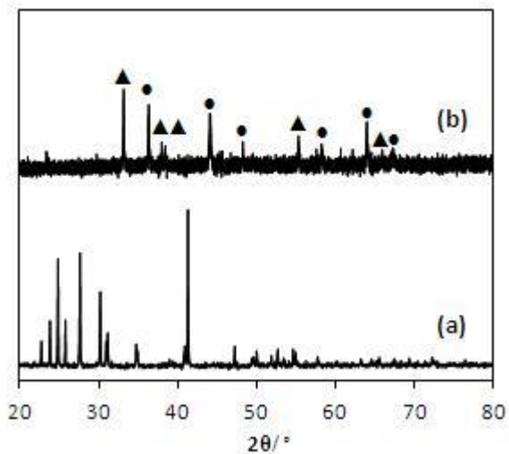
Figure 6. XRD patterns collected after the calcination step of: (a) K-Mn-O, (b) Li-Mn-O: ( \blacktriangle ) \text{LiO}_2 PDF number: 01-073-7127, ( \bullet ) \text{LiMn}_2\text{O}_4 (PDF number: 00-018-0736)
