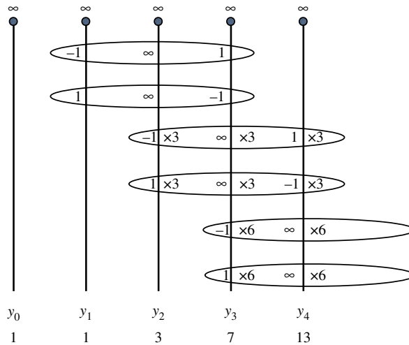
Figure 1. Calculating the degrees of the first few iterates of equation (1.4). (Online version in colour.)
