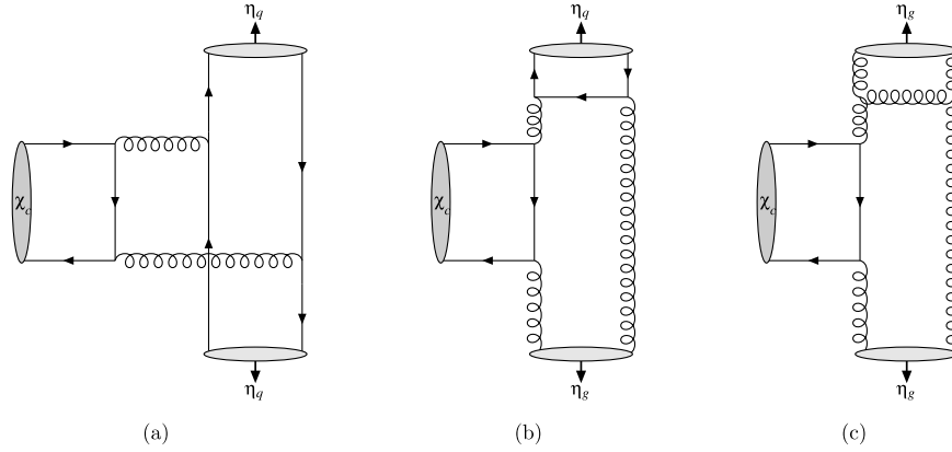
Fig. 1. Representative Feynman diagrams for \chi_c decays to \eta'(\eta') mesons, for (a) q\bar{q}q\bar{q} (b) q\bar{q}gg (c) 4g final states.
