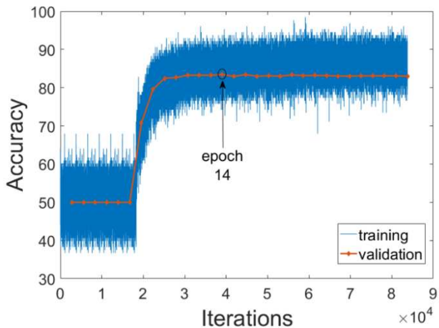
Figure 7: Plot of model accuracy on the training set (recorded at every iteration) and validation set (recorded at every epoch). Each evaluation of the gradient using the mini-batch is an iteration. The full pass of the training over the entire training set using mini-batches is an epoch.
