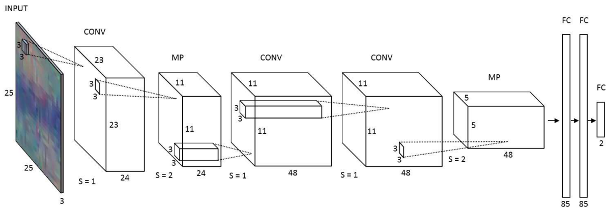
Figure 6: Schematic overview of proposed CNN architecture with respect to the convolutional (CONV), max-pooling (MP) and fully-connected (FC) layers. S = stride.
