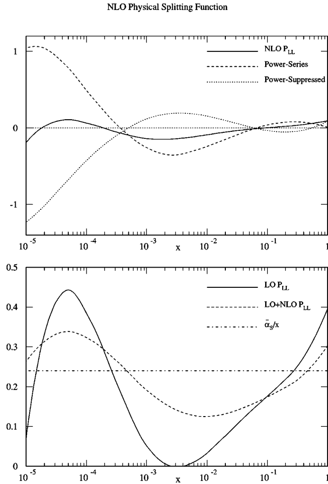
FIG. 17. (a) The splitting functions xP_{LL}^{NLO}(x) and its power-series and power-suppressed contributions plotted as functions of x for t=6 . (b) The splitting function xP_{LL}^{LO+NLO}(x) plotted as a function of x for t=6 ( Q^2 \sim 6 \text{ GeV}^2 ). Also shown is the \mathcal{O}(\alpha_s(Q^2)) contribution \bar{\alpha}_s(Q^2) , and the LO contribution xP_{LL}^{LO}(x) .
