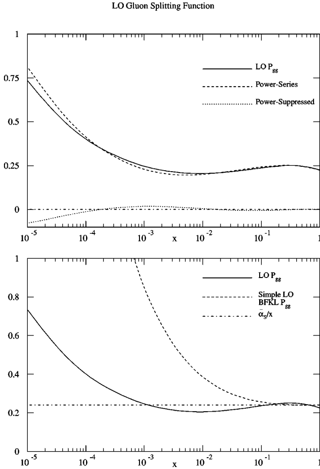
FIG. 6. (a) The splitting function xP_{gg}^{LO}(x) and its power-series and power-suppressed contributions plotted as functions of x for t = 6 . (b) The splitting function xP_{gg}^{LO}(x) plotted as a function of x for t=6 ( Q^2 \sim 6 \text{ GeV}^2 ). Also shown is the \mathcal{O}(\alpha_s(Q^2)) contribution \bar{\alpha}_s(Q^2) , and the naive LO BFKL splitting function with coupling \alpha_s(Q^2) .
