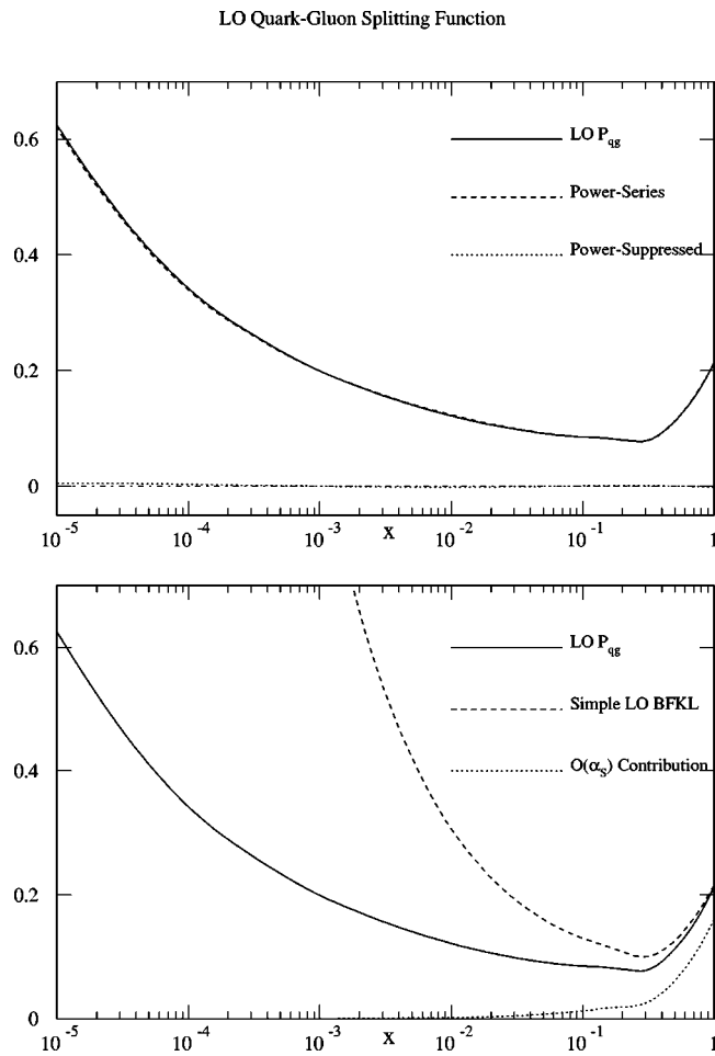
FIG. 13. (a) The full leading \ln(1/x) plus running coupling corrections coefficient function xP_{qg}(x, t) plotted as a function of x for t=6 and N_f=4 . Also shown are the contributions from the power-series and the power-suppressed part. Note that the term \propto \delta(1-x) in the power series is replaced by the full \mathcal{O}(\alpha_s(Q^2)) contribution 1.5x[x^2 + (1-x)^2] , and the terms \propto \delta(1-x) in the power-suppressed part are absent. (b) xP_{qg}^{\text{LO}}(x, t) plotted as a function of x for t=6 and N_f=4 . Also shown is the coefficient function obtained from the naive LO BFKL calculation, and the contribution at \mathcal{O}(\alpha_s(Q^2)) alone.
