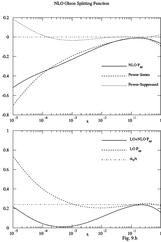
FIG. 9. (a) The splitting function xP_{gg}^{NLO}(x) and its power-series and power-suppressed contributions plotted as functions of x for t=6 . (b) The splitting functions xP_{gg}^{LO+NLO}(x) plotted as a function of x for t=6 ( Q^2 \sim 6 \text{ GeV}^2 ). Also shown is the \mathcal{O}(\alpha_s(Q^2)) contribution \bar{\alpha}_s(Q^2) , and the LO contribution xP_{gg}^{LO}(x) .
