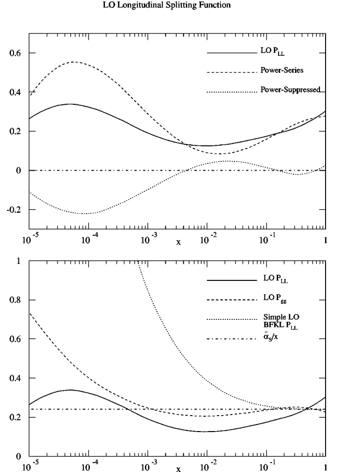
FIG. 15. (a) The splitting functions xP_{LL}^{LO}(x) and its power-series and power-suppressed contributions plotted as a function of x for t=6 . (b) The splitting function xP_{LL}^{LO}(x) plotted as a function of x for t=6 ( Q^2 \sim 6 \text{ GeV}^2 ). Also shown is the \mathcal{O}(\alpha_s(Q^2)) contribution \bar{\alpha}_s(Q^2) , the gluon splitting function P_{gg}^{LO}(x) , and the naive LO BFKL splitting function with coupling \alpha_s(Q^2) .
