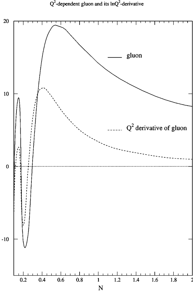
FIG. 3. The Q^2 -dependent part of the gluon structure function, \mathcal{G}_E(N,t) , and of d\mathcal{G}_E(N,t)/dt as a function of N for t=6 ( Q^2 \sim 6 \text{ GeV}^2 ). The Q^2 -independent factor of -\sin(\pi/(\bar{\beta}_0 N))\Gamma(-1/(\bar{\beta}_0 N))\exp(-\gamma_E/(\bar{\beta}_0 N)) is included in both in order to produce a smoother N -dependent normalization of the functions.
