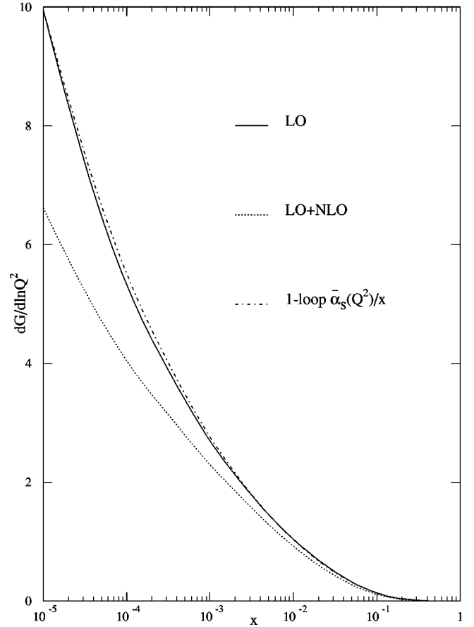
FIG. 10. The values of dG(x, Q^2)/d \ln Q^2 , for G(x, Q^2) = x^{-0.2}(1-x)^6 , due to the LO splitting function P_{gg}^{LO}(x) and the LO+NLO splitting function P_{gg}^{LO+NLO}(x) , plotted as functions of x for t=6 ( Q^2 \sim 6 \text{ GeV}^2 ). Also shown is the evolution due to the \mathcal{O}(\alpha_s(Q^2)) contribution P(x) = \bar{\alpha}_s(Q^2)/x .
