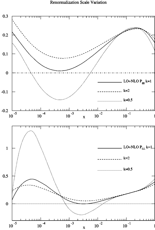
FIG. 11. (a) The renormalization scale variation of the LO+NLO splitting function P_{gg}^{LO+NLO} . Shown are the three choices of scale Q^2 , 0.5Q^2 , and 2Q^2 for t=6 , i.e. Q^2 \sim 6 \text{ GeV}^2 . (b) The same for the LO+NLO physical splitting function P_{LL}^{LO+NLO} .
