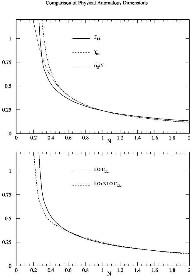
FIG. 14. (a) The anomalous dimensions for the gluon structure function at LO and for \mathcal{F}_L(N, t) at LO plotted as functions of N for t=6 . Also shown is the \mathcal{O}(\alpha_s(Q^2)) contribution common to each. (b) The anomalous dimensions for \mathcal{F}_L(N, t) at LO and “NLO” plotted as functions of N for t=6 .
