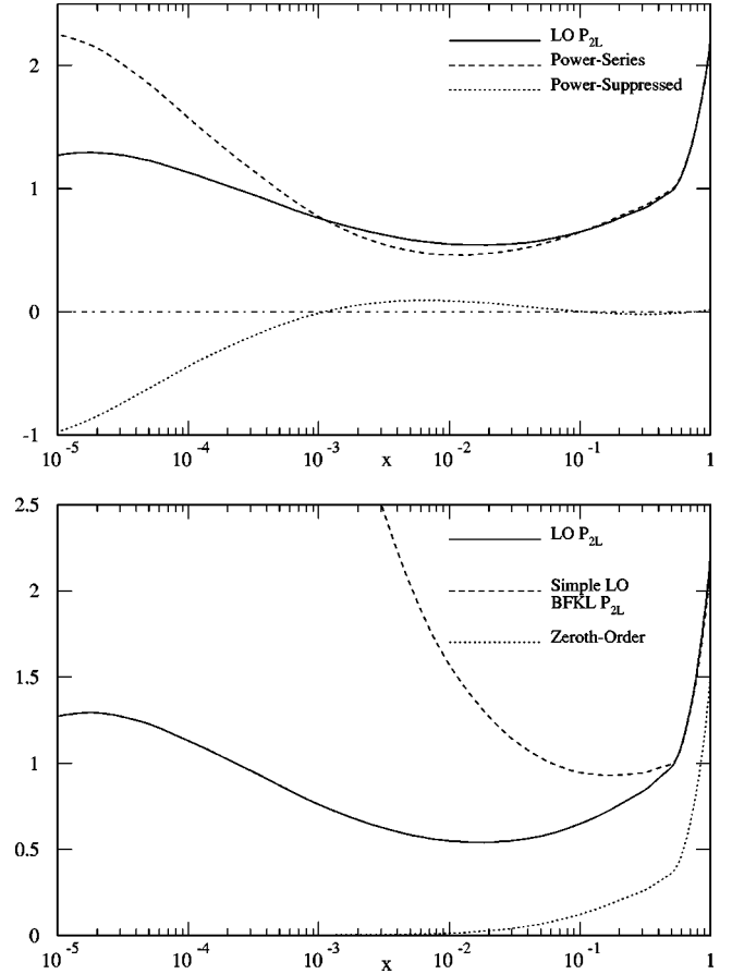
FIG. 16. (a) The full leading \ln(1/x) plus running coupling corrections physical splitting function xP_{2L}(x,t) plotted as a function of x for t=6 . Also shown are the contributions from the power-series and the power-suppressed part. In the power series the part \propto \delta(1-x) is replaced by 1.5x[x^2 + (1-x)^2] while in the power-suppressed part this contribution is simply absent. (b) The physical splitting function xP_{2L}(x,t) plotted as a function of x for t=6 along with the physical splitting function obtained from the naive LO BFKL calculation with coupling \alpha_s(Q^2) and the zeroth order contribution.
