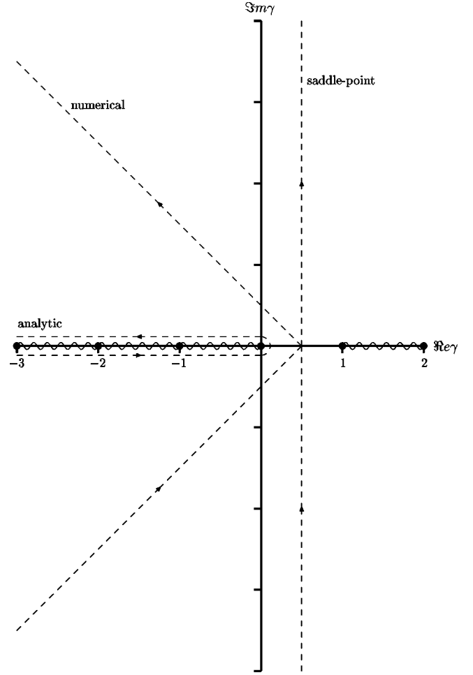
FIG. 1. The branch points and cuts associated with \exp(-X_0(\gamma)/(\bar{\beta}_0 N)) and the saddle-point contour, the gamma-function contour and the numerical integration contour.
