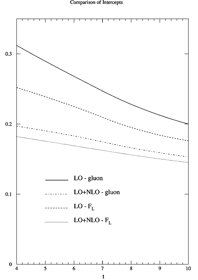
FIG. 4. The positions of the leading poles in the anomalous dimensions for the gluon structure function at LO and NLO, and for F_L at LO and NLO.
