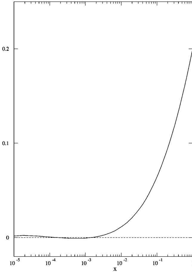
FIG. 7. The next-to-leading twist splitting function for \bar{\alpha}_s = 0.2 .
