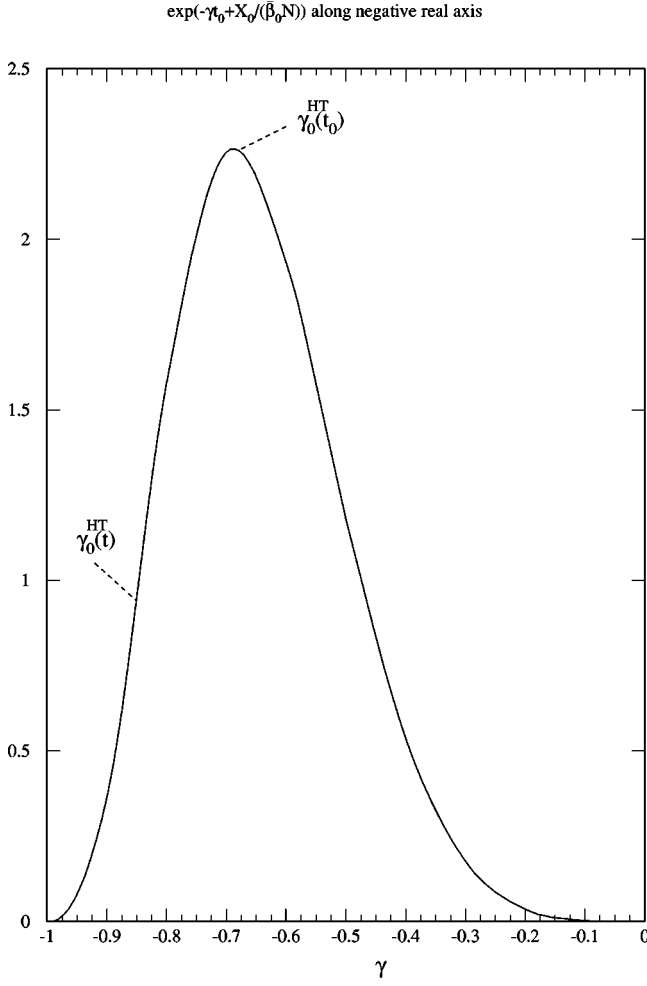
FIG. 8. The value of \exp(-\tilde{\gamma}_0 + X_0(\tilde{\gamma})/(\bar{\beta}_0 N)) , along the real axis for N=0.4 and t_0=2 , along with \tilde{\gamma} = \gamma_0^{\text{HT}}(t_0) , \gamma_0^{\text{HT}}(t) for t \gg t_0 .
