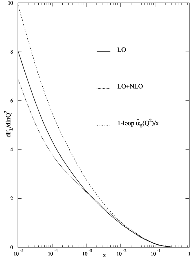
FIG. 18. The values of dF_L(x, Q^2)/d \ln Q^2 , for F_L(x, Q^2) = x^{-0.2}(1-x)^6 , due to the LO splitting functions P_{LL}^{LO}(x) and the LO+NLO splitting function P_{LL}^{LO+NLO}(x) , plotted as a function of x for t=6 ( Q^2 \sim 6 \text{ GeV}^2 ). Also shown is the evolution due to the \mathcal{O}(\alpha_s(Q^2)) contribution P(x) = \bar{\alpha}_s(Q^2)/x .
