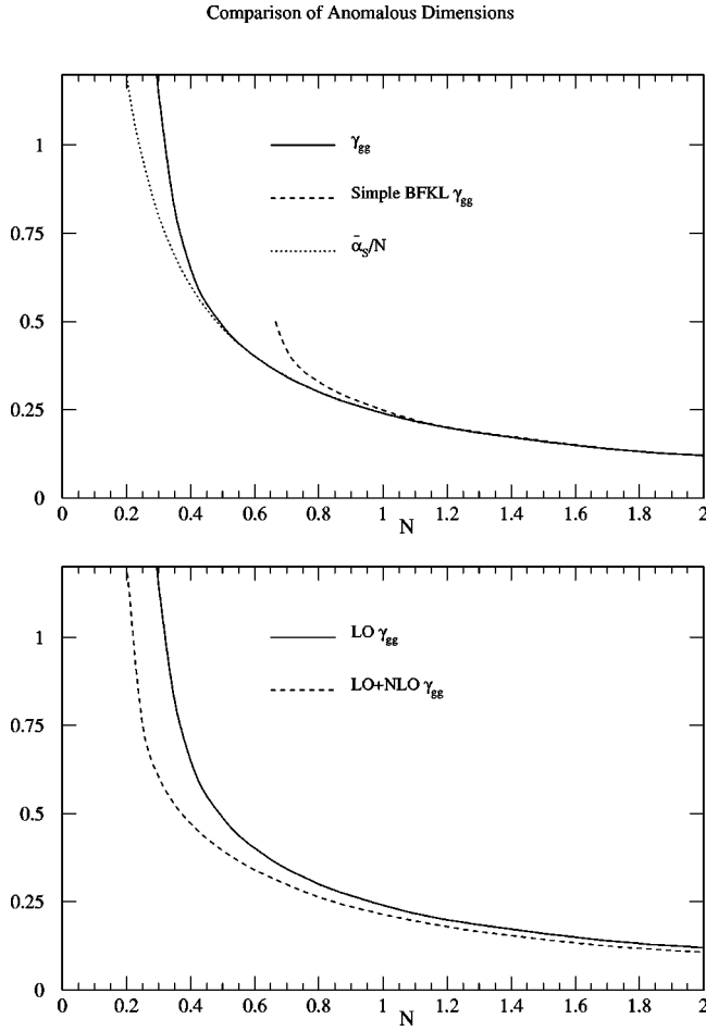
FIG. 5. (a) The anomalous dimension for the gluon structure function at LO plotted as a function of N for t=6 ( Q^2 \sim 6 \text{ GeV}^2 ). Also shown is the \mathcal{O}(\alpha_s(Q^2)) contribution \bar{\alpha}_s(Q^2)/N , and the full naive LO BFKL anomalous dimension. (b) The anomalous dimensions for the gluon at LO and at NLO plotted as functions of N for t=6 .
