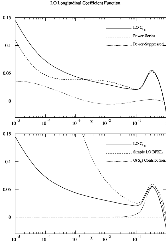
FIG. 12. (a) The full leading \ln(1/x) plus running coupling corrections coefficient function x C_{L,g}(x,t) plotted as a function of x for t=6 and N_f=4 . Also shown are the contributions from the power-series and the power-suppressed part. Note that the term \propto \delta(1-x) in the power series is replaced by the full \mathcal{O}(\alpha_s(Q^2)) contribution 6x^2(1-x) , and the terms \propto \delta(1-x) in the power-suppressed part are absent. (b) x C_{L,g}^{LO}(x,t) plotted as a function of x for t=6 and N_f=4 . Also shown is the coefficient function obtained from the naive LO BFKL calculation, and the contribution at \mathcal{O}(\alpha_s(Q^2)) alone.
