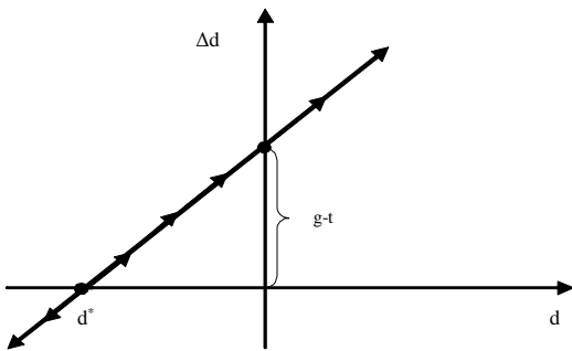
Phase diagram 3
