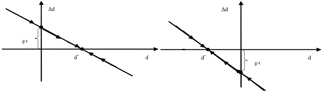
Phase diagram 1
