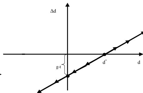
Phase diagram 4
