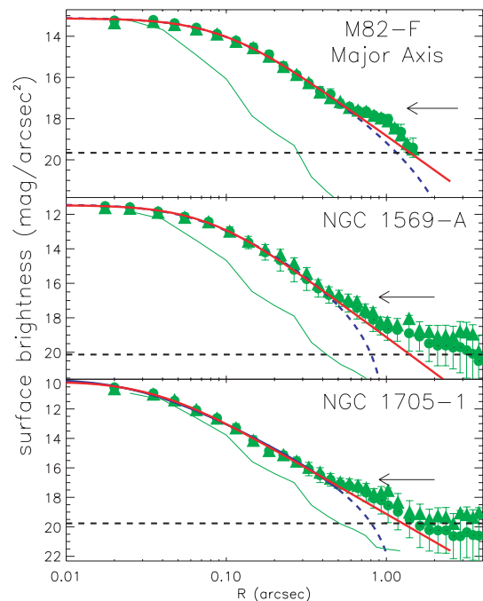
Figure 1. The luminosity profiles of the young massive clusters M82-F, NGC 1569-A and NGC 1705-1. The data are shown as filled green symbols, where the circles are the mean of the flux at that radius and the triangles are the median of the flux. Error bars represent the standard deviation of pixels in that annulus (based on the mean flux). The PSF is shown as a solid green line and the background value is the horizontal dashed line. The best-fitting King (blue/dashed) and EFF (red/solid) profiles are shown – see text. The fits were carried out for R < 0.5 arcsec. Note that all clusters contain excess light at large radii relative to either of the profiles; the break from the EFF profile is denoted by an arrow.
