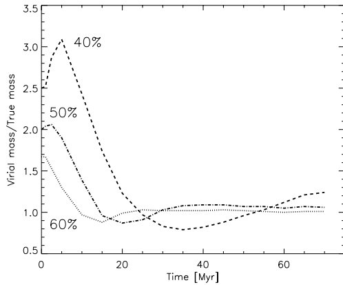
Figure 3. The variation of the virial-mass-to-true-mass ratio with time for effective star formation efficiencies of 40, 50 and 60 per cent. The virial mass is measured from the velocity dispersion of stars within 20 pc of the cluster centre and the true mass is the total mass of stars within 20 pc of the cluster. Note that zero time is the time of gas expulsion, and so the cluster age is \sim 5 Myr greater than this time.
