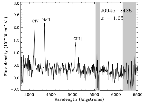
Figure 1. The 1D spectrum of the type II quasar, J0945-2428 at z = 1.65 . The spectrum was extracted over the whole galaxy (seven IFU fibres). The shaded regions show the wavelengths affected by sky line emission.
