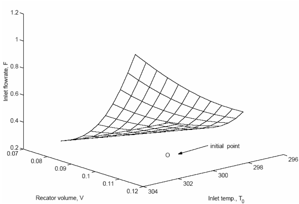
Fig. 4. Locus of input multiplicity condition between the inlet flow rate, inlet temperature and reactor volume
