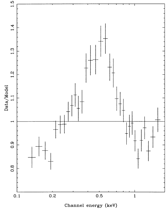
Figure A2. Ratio of a power-law model (best-fitting \Gamma = 2.2 ) with fixed Galactic N_H , to the P9 spectrum after correction with PCPICOR. Note that the residuals now have a similar shape to those in Fig. 4.
