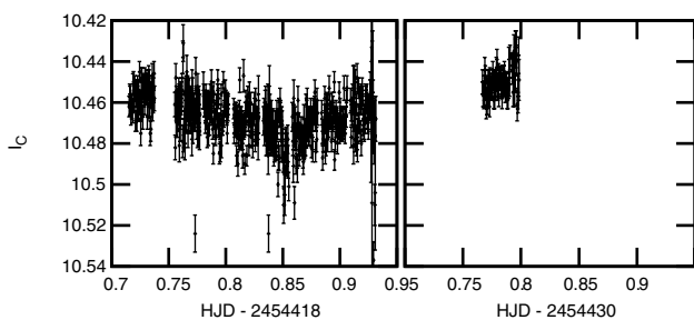
Figure 3. Cousins I_C -band photometric data provided by observer CTX.
