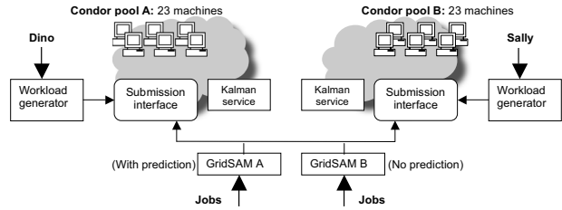
Figure 5. Test-bed Architecture.
