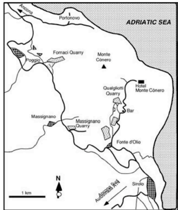
Figure 1. Location of the Fonte d'Olio section at Monte Cònero (from Montanari & Koeberl, 2000).
