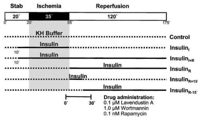
Figure 1. Experimental protocol. Stab indicates stabilization; dotted lines, buffer perfusion; solid lines, insulin infusion; Ins_{I,I} , insulin administration for the last 10 minutes of stabilization and for the duration of ischemia; Ins_{I,I+R} , insulin for 10 minutes prior to ischemia, during ischemia and reperfusion; Ins_{R,I} , insulin during reperfusion; Ins_{R,I+15} , insulin for the 15 first minutes of reperfusion; Ins_{R,-15} , insulin infusion started 15 minutes after the onset of reperfusion. The inhibitors (lavendustin A, wortmannin, and rapamycin) were administered for 30 minutes; from 30 minutes of ischemia until 25 minutes of reperfusion.
