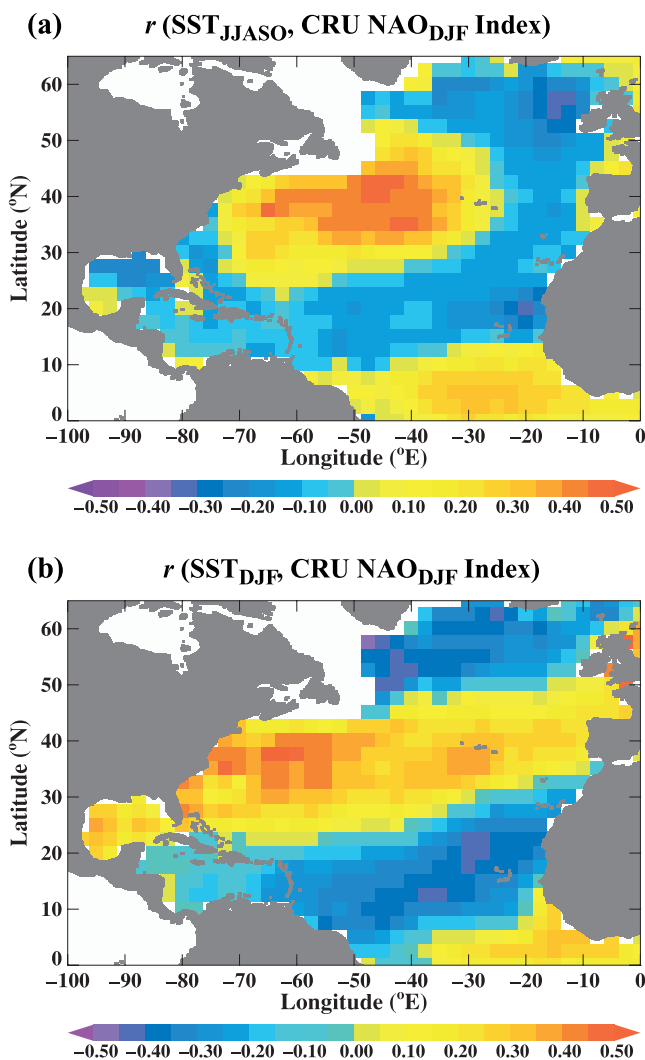
Figure 2. The correlation patterns of north Atlantic (a) SST_{JJASO} and (b) SST_{DJF} anomalies with the CRU NAO_{DJF} index for the period 1950/1–2000/1. Correlation values of 0.28, 0.36 and 0.45 are significant respectively at the levels 0.05, 0.01 and 0.001.
