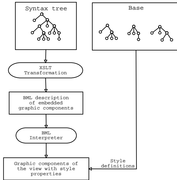
Fig. 18. Schema of graphical view construction
