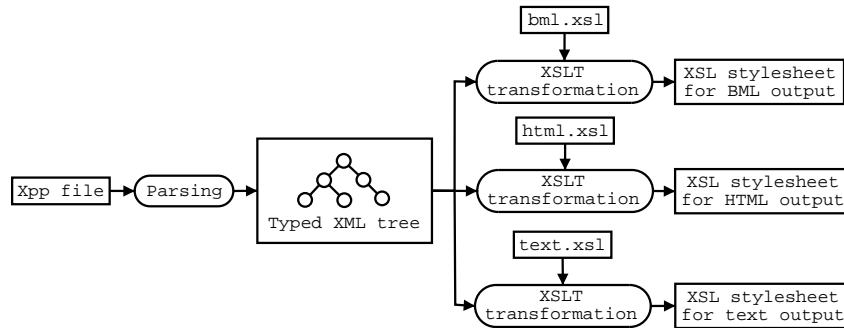
Fig. 21. From Xpp to XSLT
