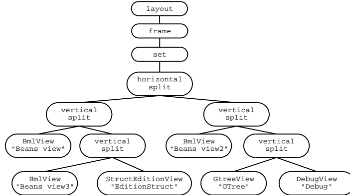
Fig. 23. Schematic graph of the AST in Figure 22
