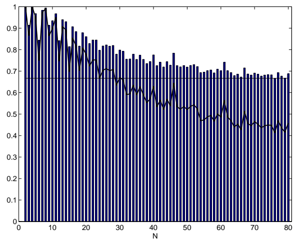
FIG. 2: The bar plot shows the maximum fidelity F of quantum communication and the curve shows the maximum sharable entanglement \mathcal{E} achieved in a time interval [0, 4000/J] as a function of the chain length N from 2 to 80. The time t_0 at which this maxima is achieved varies with N . The straight line at F = 2/3 shows the highest fidelity for classical transmission of a quantum state.
