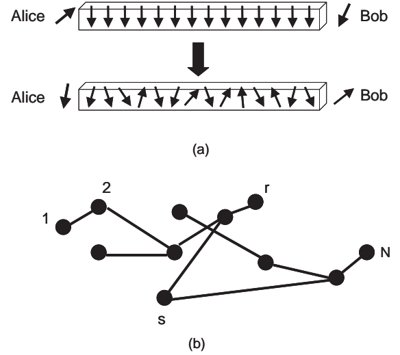
FIG. 1: The part (a) of the figure shows our quantum communication protocol. Initially the spin chain is in its ground state in an external magnetic field. Alice and Bob are at opposite ends of the chain. Alice places the quantum state she wants to communicate on the spin nearest to her. After a while, Bob receives this state with some fidelity on the spin nearest to him. Part (b) shows an arbitrary graph of spins through which quantum communications may be accomplished using our protocol. The communication takes place from the sender spin s to the receiver spin r .
