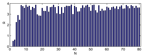
FIG. 3: The upper part plots \alpha = \log_{10} 2Jt_0 where t_0 is a time in the interval [0, T_{max} = 4000/J] when the maximum fidelities F plotted in fig2 are achieved.
