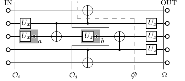
FIG. 4: Vertical cuts. The vertical cuts intersect each qubit line exactly once but do not intersect gates. Thus, \mathcal{O}_i , \mathcal{O}_j and \Omega are vertical cuts, but \mathcal{O} is not. The cut \mathcal{O}_i intersects the rotation U_x just before its input. For two of the rotations in the displayed network, the sub-clusters on which these gates are realized are symbolically displayed in gray underlay. Via the measurement of the cluster qubits a and b (displayed as black dots with white border), the rotation angles of the respective rotations U_x and U_z are set.
