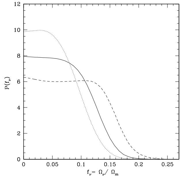
FIG. 3. Probability distributions, normalized so that the area under each curve is equal to 1, for f_\nu with marginalization over the other parameters, as explained in the text, for N_\nu = 3 massive neutrinos and n = 0.9 (dotted line), 1.0 (solid line), and 1.1 (dashed line).
