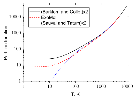
Figure 11. A comparison between the partition function produced from our line list and the theoretical partition function described by Sauval & Tatum (1984). The latter values were multiplied by g_{ns} = 2 .
