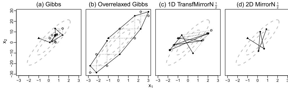
Figure 8: Sample path from a few steps of four algorithms for sampling from N_2(0, \Sigma) , with \Sigma = \begin{pmatrix} 1 & 9 \\ 9 & 100 \end{pmatrix} : (a) standard Gibbs sampler, (b) overrelaxed Gibbs sampler ( \alpha = -0.98 ), (c) MH using 1D TransfMirrorN _{\frac{1}{2}} kernel, and (d) MH using 2D MirrorN _{\frac{1}{2}} kernel. The first three consist of a sequence of two one-dimensional moves, while the last one is a single two-dimensional move. The 1D TransfMirrorN _{\frac{1}{2}} kernel applies the MirrorN kernel y'_i | y_i \sim N(2(\hat{\Sigma}^{-1/2} \mu^*)_i - y_i, \frac{1}{4}) , i = 1, 2 , on y = \hat{\Sigma}^{-1/2} x , where x = (x_1, x_2) is the target variable, and \mu^* and \hat{\Sigma} are estimated mean and covariance matrix of the target from the burn-in as described in Section 4.2. The 2D MirrorN _{\frac{1}{2}} kernel proposes x' | x \sim N(2\mu^* - x, \frac{1}{4} \hat{\Sigma}) . Triangle = starting point (-1, 4) ; filled circle = state of the Markov chain; empty circle = intermediate step (for the one-dimensional moves). Two ellipses enclose the 50% and 90% probability mass of the target.
