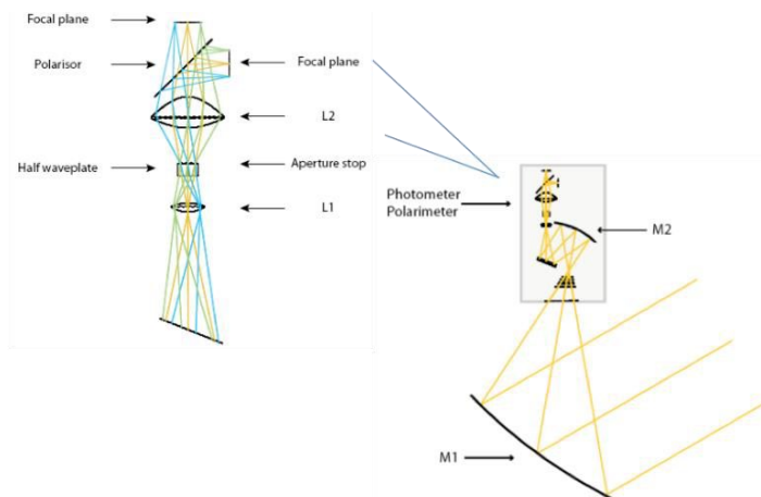
Fig. 1. PILOT Optical Layout. Only the M1 mirror is located outside the photometer.
