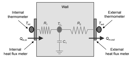
Figure 1: Schematic of the wall and one-dimensional heat transfer assumption (black arrows).
