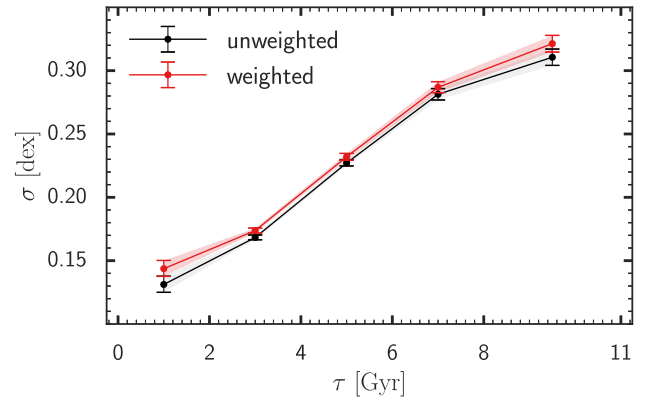
Figure 8. The best-fitting estimates and their uncertainties for the dispersion, \sigma , for our vertical metallicity gradient fitting for mono-age stellar populations as a function of age, \tau , in both the weighted (light red) and unweighted (black) cases. The shaded area gives the uncertainty space of the dispersion in the unweighted case.
