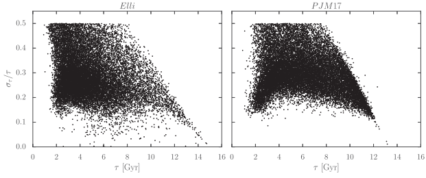
Figure A2. Fractional age uncertainty as a function of age for both the ‘ Elli ’ sample and ‘ PJM17 ’ sample (see text).
