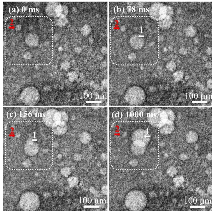
Fig. 5. Nucleation and fast growth of a single cavitation gas bubble: (a) just before nucleation; (b) <78 ms after the nucleation process starts and is represented by the light dotted area on top left region of the bubble's periphery (white arrow); (c) in growth process; (d) the end of growing process at the end of cycle (1.0 s).
