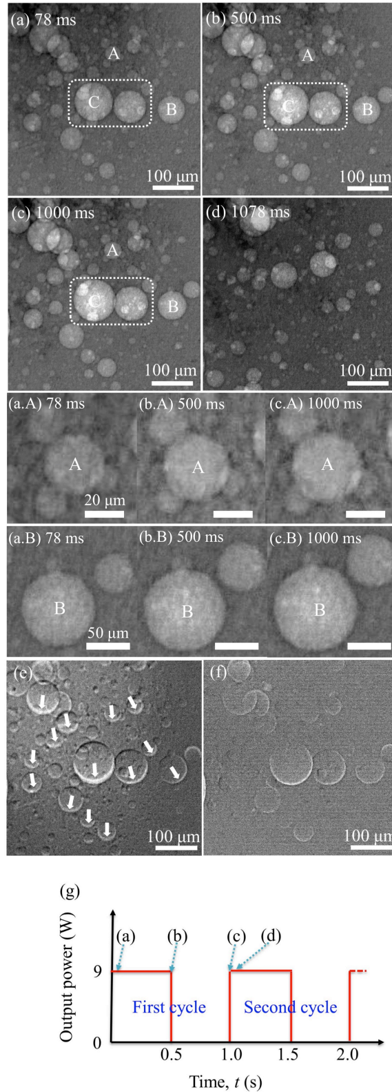
Fig. 2. Typical behaviour of cavitation bubbles under present sonication conditions (see Table I): (a) 78 ms after the start of sonication; (b) sonication stops at 500 ms; (c) end of cycle (1000 ms); (d) 78 ms after the start of a new cycle; (e) image difference by subtracting frame
