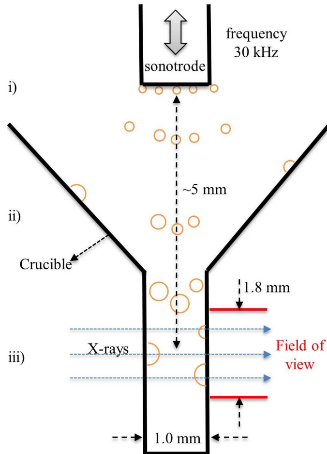
Fig. 3. Sketch map of cavitation gas bubble activities under current ultrasonication (Table I): i) bubble generation in cavitation zone (region close to the sonotrode tip); ii) bubble travelling downwards towards the bottom of the crucible; iii) bubble attachment onto the inner surface of the container, some of which are located within the field of view where X-rays are passing through the melts. A number of key dimensions are indicated.
