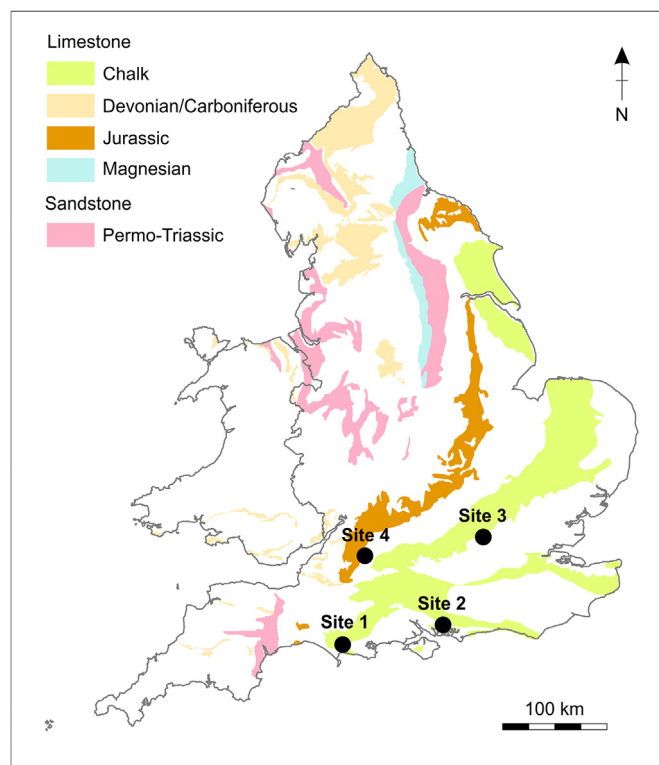
Fig. 1. Location of public water supplies and major aquifers of the UK. Note the Portland Stone Formation is too small to be visualised at this scale.
