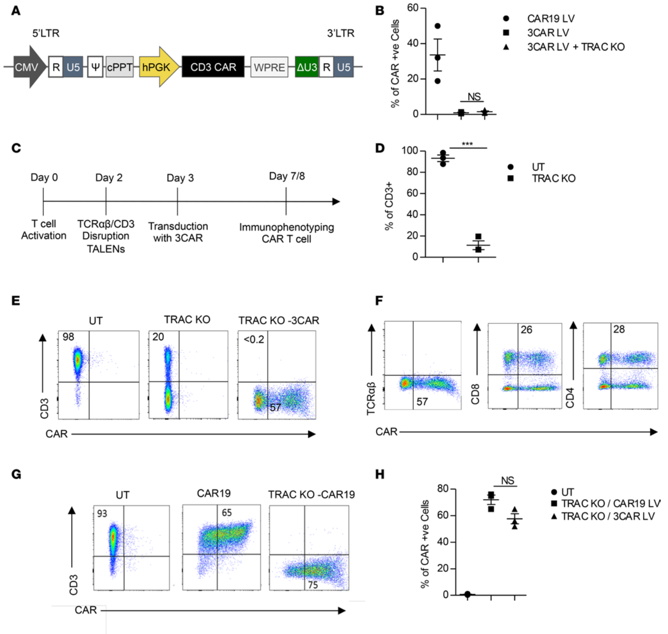
Figure 1. Successful generation of 3CAR requires disruption of CD3ε expression prior to lentiviral 3CAR transduction. (A) Vector configuration showing codon optimized single-chain variable fragment (scFv) derived from OKT3 with CD8 stalk and 41BB/CD3ζ activation domains, all under the control of an internal human phosphoglycerate kinase (hPGK) promoter in a third-generation self-inactivating (SIN) lentivirus with HIV-1-derived reverse response element (RRE), central polypurine tract (cPPT), and mutated woodchuck hepatitis virus posttranscriptional regulatory element (WPRE). Human cytomegalovirus (CMV); Repeat region (R); Unique 5' region (U5); Psi (Ψ); and modified unique 3' region (ΔU3). (B) Percentage of CAR + cells with and without TRAC-KO prior to lentivirus (LV). Data are presented as mean ± SEM. n = 3 donors. (C) Schema of event precedence required for successful 3CAR T cell production. CD3/CD28 activation with TransAct for 48 hours was followed by electroporation of mRNA encoding TRAC-specific TALENs ahead of LV transduction by 72 hours. (D) Summary of CD3 + cells following TRAC-KO ( n = 3 donors), mean ± SEM. *** P < 0.0005, by unpaired, 2-tailed Student's t test. (E) Representative flow cytometry plots of day 7 cells. In cultures with 3CAR expression, there were no surviving CD3 + cells compared with 20% residual expression in the absence of 3CAR transduction ( n = 3 donors). (F) Representative flow cytometry plots showing 3CAR T cells retained CD4 and CD8, but not TCRαβ, expression; n = 3 donors. (G) For comparison, control transductions with LV CAR19 mediated 65% transduction but required further processing by column-mediated TCRαβ depletion to yield TRAC-KO CAR19 + T cells; n = 3 donors. (H) Summary of CAR + cells following TRAC-KO ( n = 3 donors); mean ± SEM. Two-tailed Student's t test.
