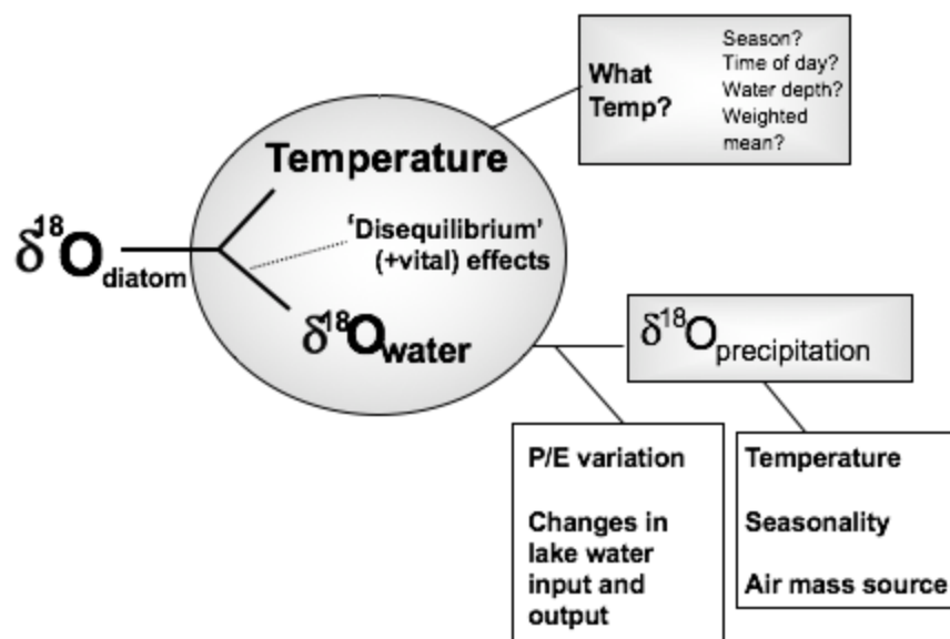
116 117 Fig. 1: Controls on the stable oxygen isotope composition of biogenic silica
