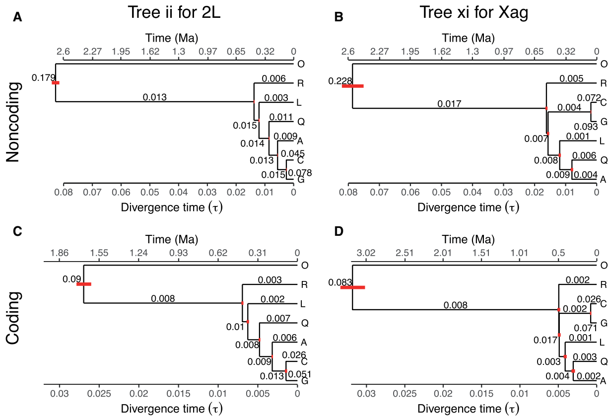
Fig. 2. Trees ii and xi with posterior estimates of population sizes ( \theta s, numbers on the branches) and species divergence times ( \tau s, the bottom horizontal axis; bars represent 95% HPD intervals) from BPP. Parameters for tree ii were estimated from all loci in chromosome 2L excluding 2La region, while those for tree xi were estimated from all loci in the Xag region of chromosome X. Divergence times were calculated assuming the mutation rate 2.8 \times 10^{-9} per site per generation for autosomal noncoding loci (A), with 11 generations per year, and 0.524 and 0.323 times (supplementary fig. S4, Supplementary Material online) as large for the coding autosomes (C) and coding Xag loci (D), respectively. Ma, million years ago.
