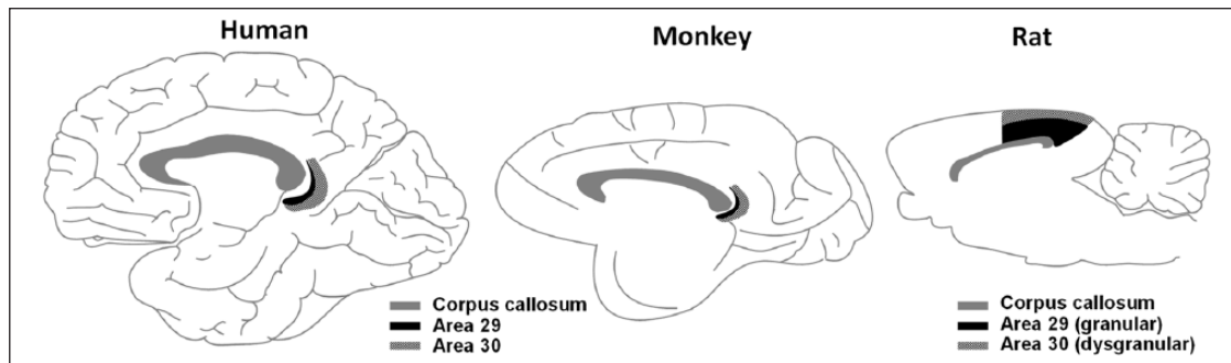
Figure 1. Schematic of the RSC as seen in midsagittal section and located just posterior to the corpus callosum, in humans, rhesus monkeys and rats. Source: Figure by Jeffery (2017); available at: https://doi.org/10.6084/m9.figshare.5414179.v1 under a CC-BY 4.0 licence.
