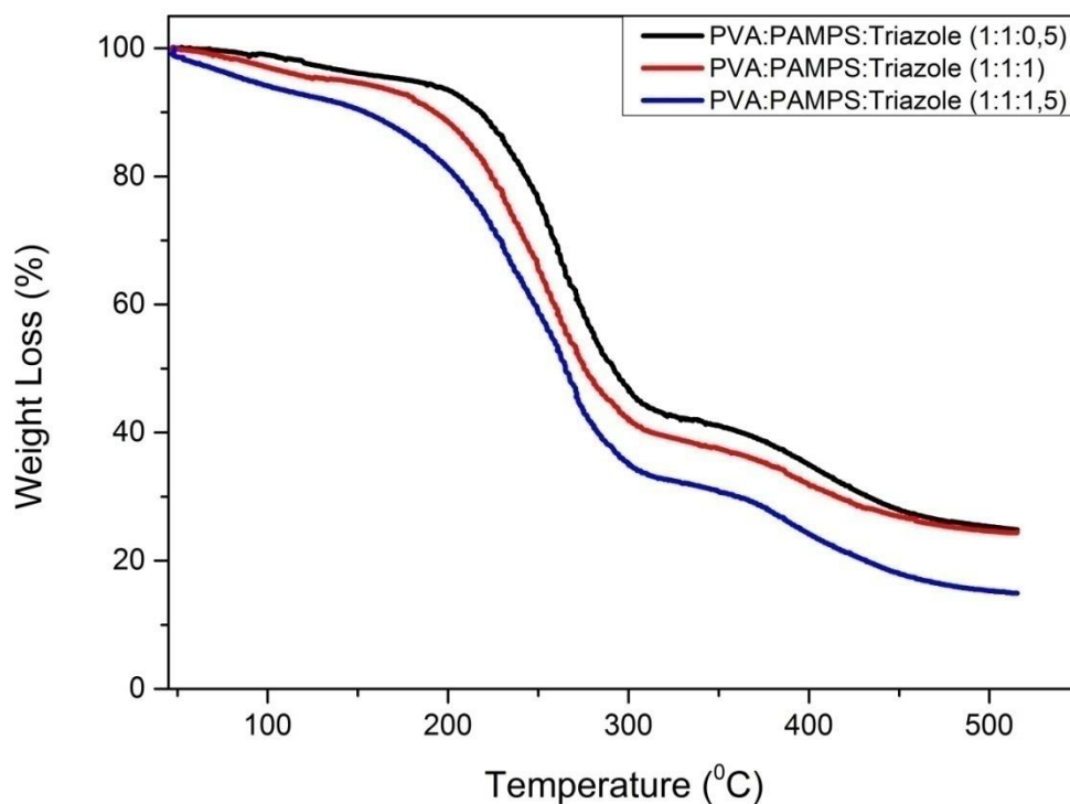
Fig. 5. Thermogravimetric (TGA) thermographs of the composite membranes.
