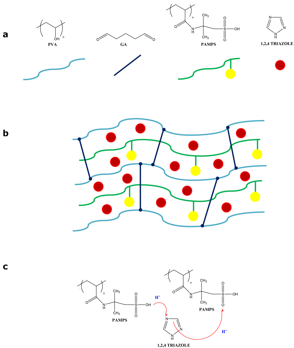
Fig. 2a. The chemical structures of PVA, GA, PAMPS, and 1,2,4-triazole. 2b. The proposed membrane microstructure for the cross-linked PVA/PAMPS/1,2,4-triazole. 2c. The proposed proton transfer path along PAMPS chains and 1,2,4-triazole molecules.
