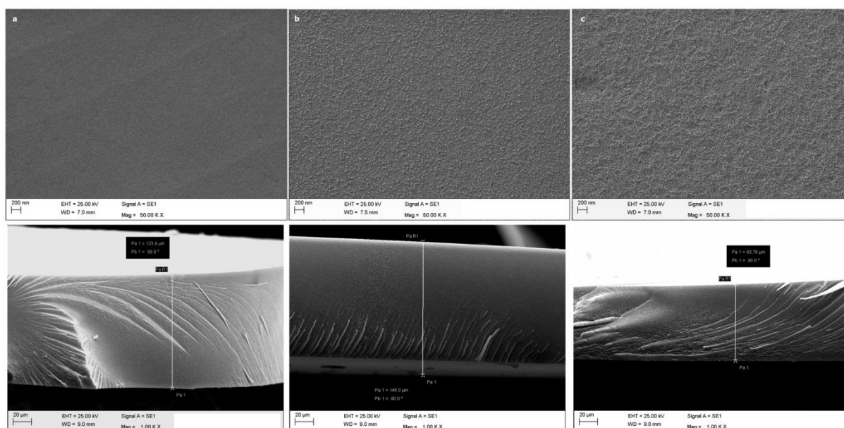
Fig. 4. Surface and cross-sectional SEM micrographs of the composite membranes with different 1,2,4-Triazole compositions: (a) PVA:PAMPS:Triazole (1:1:0.5), (b) PVA:PAMPS:Triazole (1:1:1), and (c) PVA:PAMPS:Triazole (1:1:1.5)
