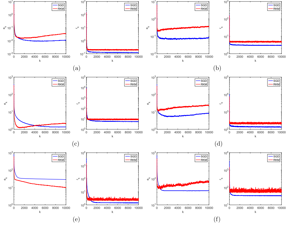
Figure 5. Numerical results for the examples by SGD (with \alpha = 0.1 ) and RKM. (a) phillips, \delta = 10^{-2} . (b) phillips, \delta = 5 \times 10^{-2} . (c) gravity, \delta = 10^{-2} . (d) gravity, \delta = 5 \times 10^{-2} . (e) shaw, \delta = 10^{-2} . (f) shaw, \delta = 5 \times 10^{-2} .
