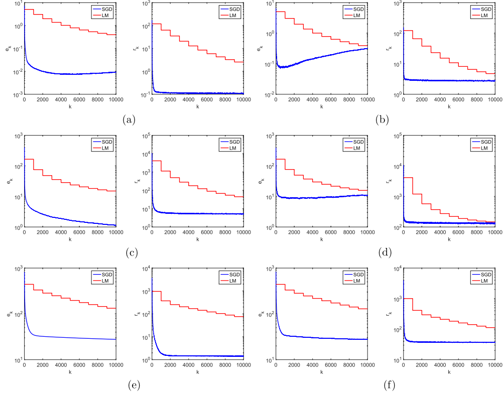
Figure 4. Numerical results for the examples by SGD (with \alpha = 0.1 ) and LM. (a) phillips, \delta = 10^{-2} . (b) phillips, \delta = 5 \times 10^{-2} . (c) gravity, \delta = 10^{-2} . (d) gravity, \delta = 5 \times 10^{-2} . (e) shaw, \delta = 10^{-2} . (f) shaw, \delta = 5 \times 10^{-2} .
