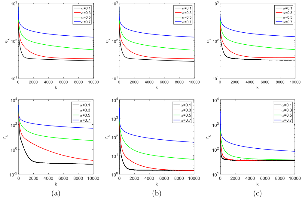
Figure 3. Numerical results for shaw with different noise levels by SGD (with various \alpha ). (a) \delta = 1 \times 10^{-3} . (b) \delta = 1 \times 10^{-2} . (c) \delta = 5 \times 10^{-2} .
