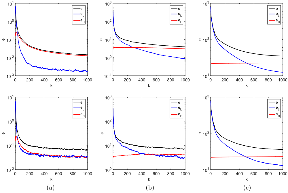
Figure 6. The error decay for the examples with two noise levels: \delta = 10^{-2} (top) and \delta = 5 \times 10^{-2} (bottom), with a truncation level L = 5 . (a) phillips. (b) gravity. (c) shaw.
