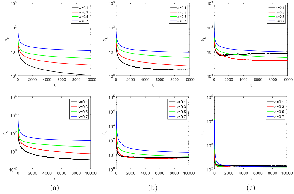
Figure 2. Numerical results for gravity with different noise levels by SGD (with various \alpha ). (a) \delta = 1 \times 10^{-3} . (b) \delta = 1 \times 10^{-2} . (c) \delta = 5 \times 10^{-2} .
