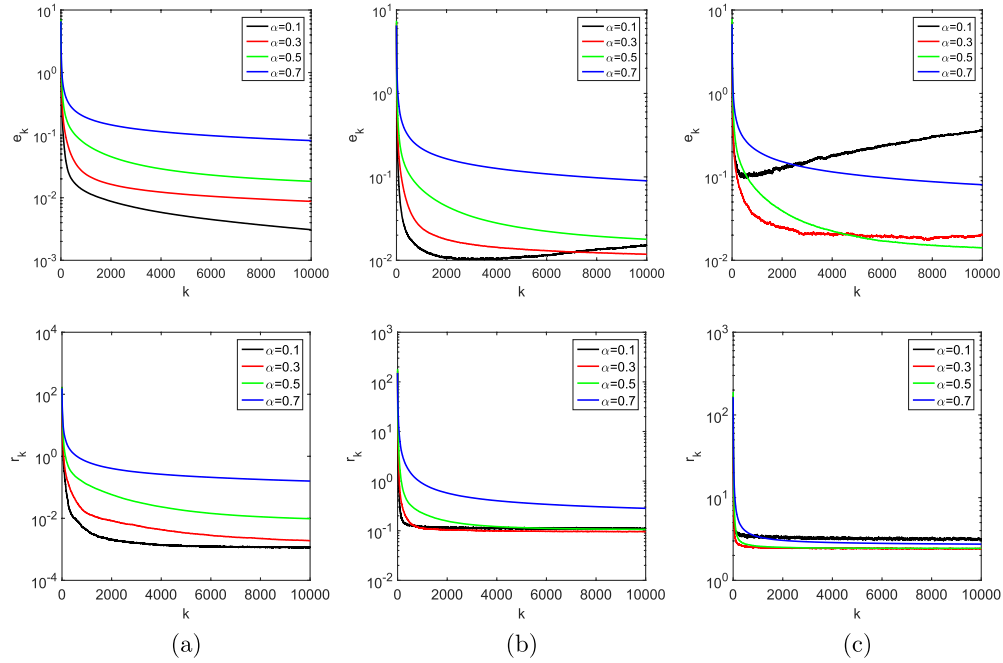
Figure 1. Numerical results for phillips with different noise levels by SGD (with various \alpha ). (a) \delta = 1 \times 10^{-3} . (b) \delta = 1 \times 10^{-2} . (c) \delta = 5 \times 10^{-2} .
