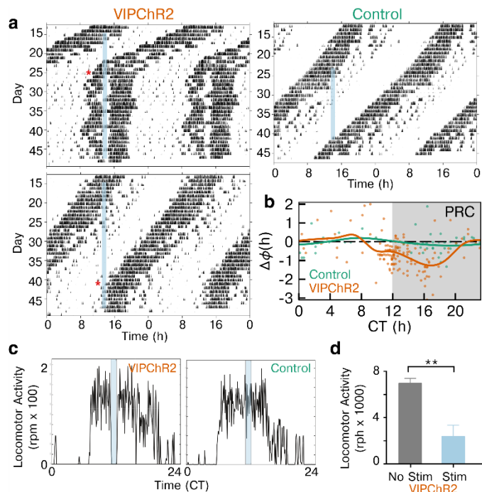
Figure 5. Stimulation of VIP neurons in vivo entrains locomotor activity. a) Daily locomotor activity of two representative mice entrained to HIF stimulation of SCN VIP neurons (blue bar) compared to a control mouse lacking ChR2. Actograms show wheel revolutions per 6 min (black bars) recorded from enucleated mice for almost 50 days. Note that the two VIPChR2 mice, with slightly different periods, reached stable entrainment (*) only when the stimulation occurred around early subjective night. b) Average phase response curves following stimulation of VIPChR2 (orange, n = 7) and control mice (green, n = 4) show the change in phase (dots) on the day after stimulation at different circadian times. Note that activation of VIP neurons entrained daily locomotor rhythms primarily through phase delays when delivered during the late subjective day and early subjective night. c) Representative activity profiles of 2 mice show that HIF stimulation of VIP neurons acutely reduced running wheel activity in VIPChR2 (left), but not control (right), mice. d) Wheel revolutions during optogenetic stimulation (CT 12-18, 1 h of HIF) decreased nearly four-fold compared to baseline in VIPChR2 mice ( 2355.0 \pm 981.1 during stimulation vs. 6958.0 \pm 418.9 with no stimulation, n = 6 mice, paired Student's t-test **p < 0.01 ).
