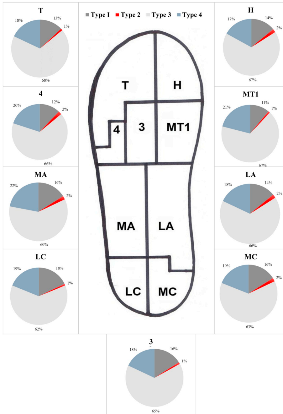
Fig. 5. Mean spatial distribution of the different quartz grain types across the soles of the shoes in Study 1.
