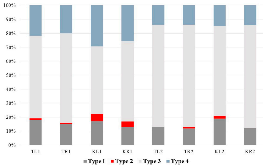
Fig. 4. The percentage of grain types present on each shoe sole during Study 1.
