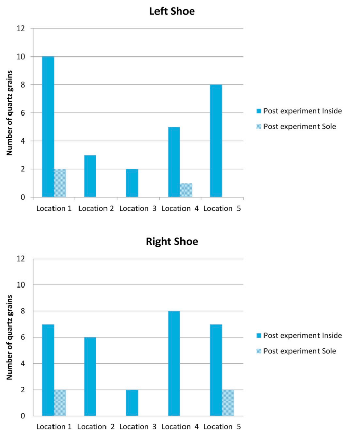
Fig. 8. Graph to illustrate the quartz grain types present inside and on the sole of the footwear at the end of Study 2.
