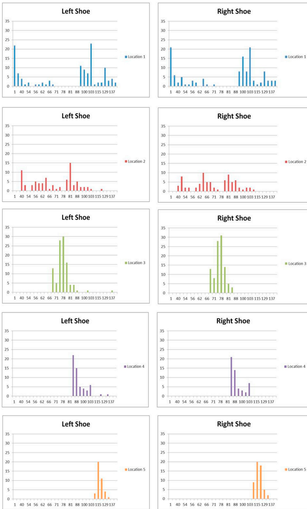
Fig. 7. Graphs to illustrate the persistence of quartz grain types on footwear soles during Study 2. For each graph y-axis: number of grains, x-axis: number of days.
