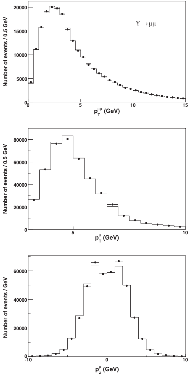
FIG. 14. Distributions of p_T^{\mu\mu} (top), p_T^\mu (middle), and p_z^\mu (bottom) in the data (circles) and the tuned simulation of \Upsilon decays (histogram). The data distributions correspond to the mass range 9.30–9.56 GeV and are background-subtracted using events in the mass ranges 9.17–9.30 and 9.56–9.69 GeV.
