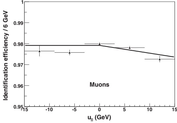
FIG. 6. Muon identification efficiency as a function of the recoil component in the direction of the muon ( u_{\parallel} ).
