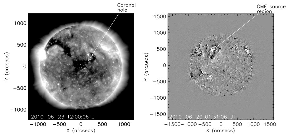
Figure 1. (left) AIA/SDO image of the solar disk on 23 June 2010 in the 193 Å passband. The coronal hole labeled is the source of the high-speed solar wind stream which causes the CIR. (right) Running difference EUVI-B image at 01:30 UT showing the CME source location.
