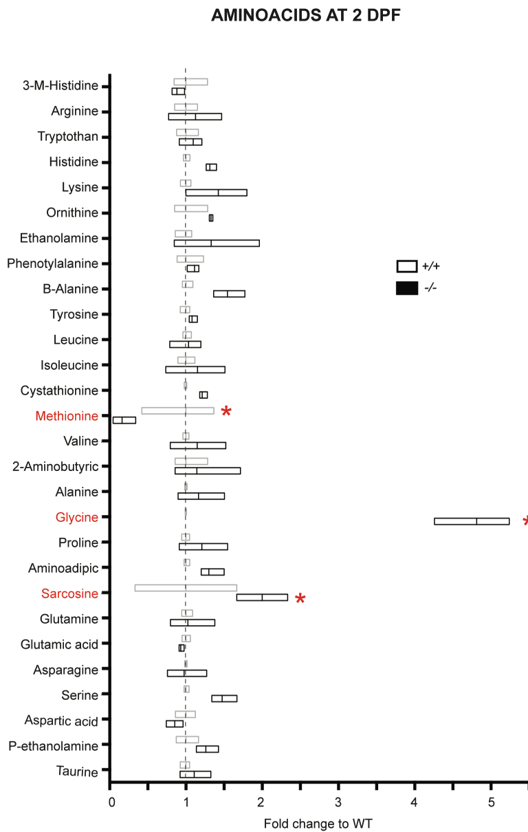
Supplemental Figure 1: LC-MS analysis of the levels of the main proteogenic and non-proteogenic amino acids at 2 dpf reveals a significant increase in sarcosine and glycine as well as a decrease in methionine level between glc -/- and +/+ embryos. Box and whiskers display min and max values and a line shows the median value.
