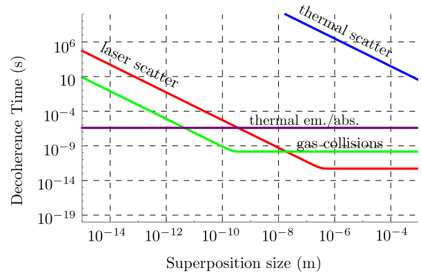
Figure 3: Decoherence times from continuous measurement by the trapping laser for the example of a superposition state: The decoherence time due to laser light scattering (red line) is estimated using Eq. (27). We have plotted for comparison the decoherence time due to emission and absorption of thermal photons (purple line), where we have assumed that the internal and external temperatures are the same, namely at 300 K, scattering of thermal photons (blue line) and gas collisions (green line) at a background gas pressure of 10^{-2} mbar [42–44].
