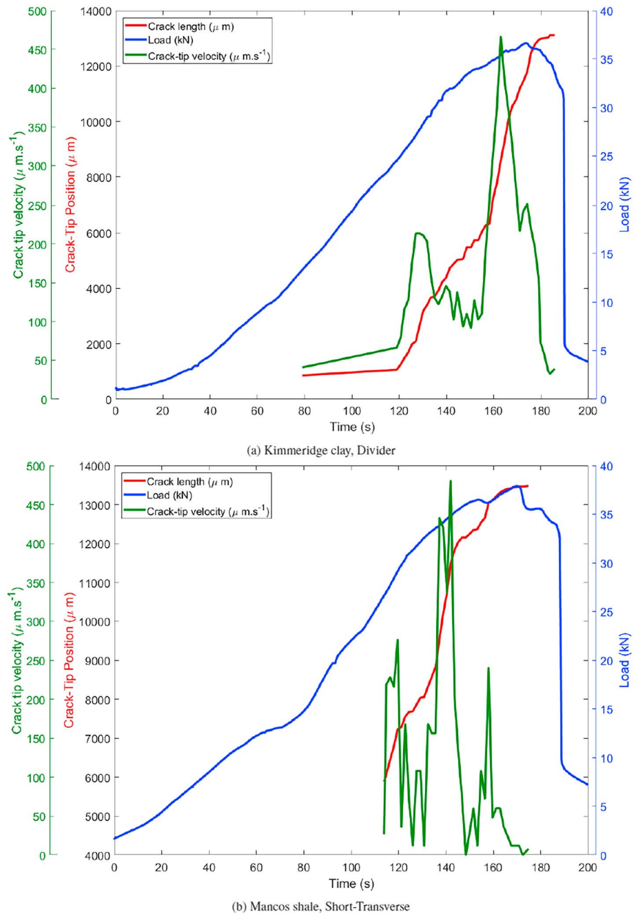
Figure 8. Crack-tip position, velocity, and load as a function of time for a Divider orientation sample of Kimmeridge clay (a), and a Short-Transverse orientation sample of Mancos shale (b). Crack-tip position and velocity are measured exclusively in the y direction as defined in Figure 2. The velocity data has a 5-point moving average filter applied.
