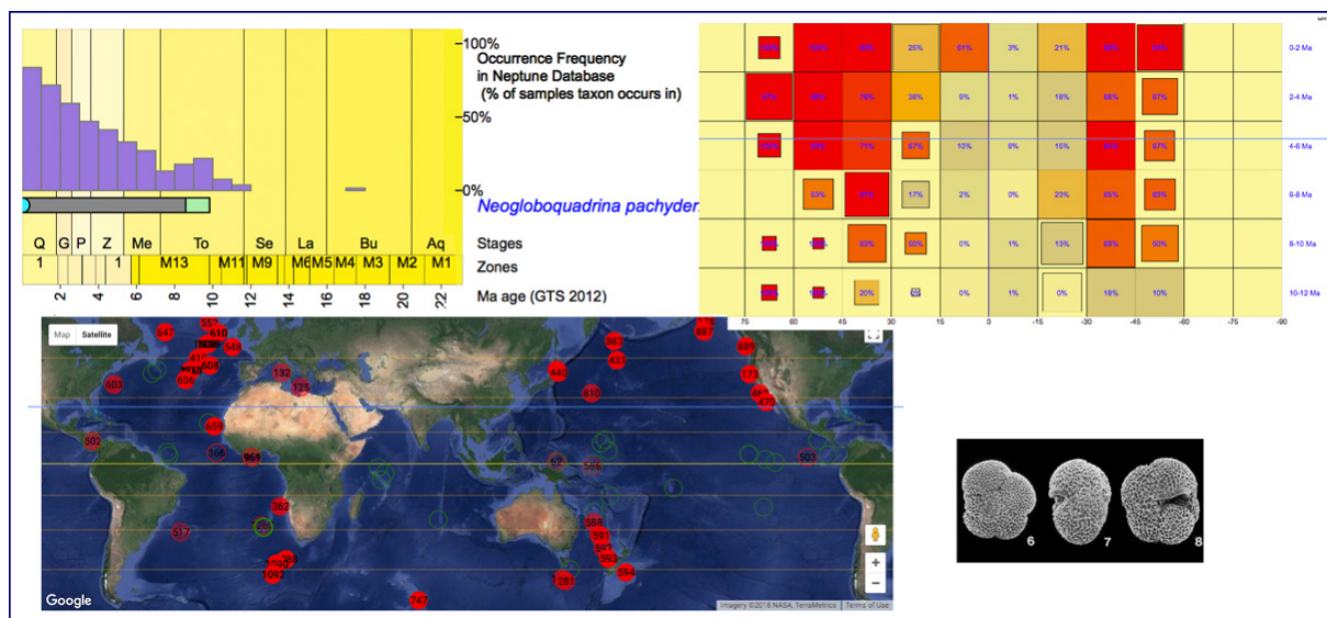
Fig. 3. Display of occurrence data from Neptune database for a single species Neogloboquadrina pachyderma
