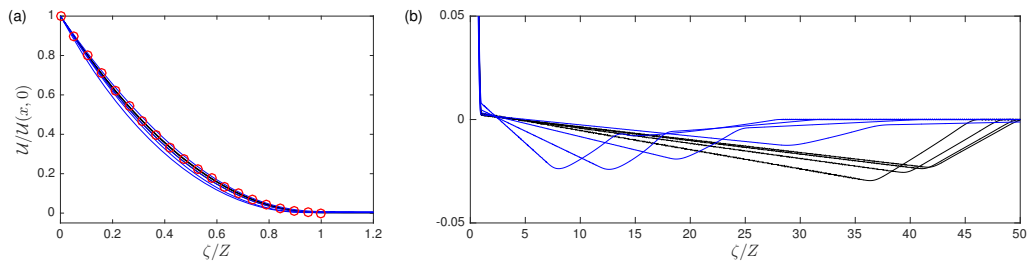
FIGURE 13. Boundary-layer horizontal velocity profiles in a stationary frame for a = 0.3 and \text{Bi} = 512 . Profiles, scaled by the velocity of the wave \mathcal{U}(x, 0) , are taken at x = 0, 0.1, 0.2, 0.3 (black) and x = 0.7, 0.8, 0.9, 1 (blue), and compared with the theoretical prediction in (4.12) (red circles). (a) A large-scale plot of the boundary layer against the swimmer; (b) the same data on a larger scale, showing the gently rotating plugs above the boundary layer (where the scalings do not collapse all the curves).
