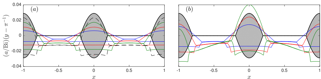
FIGURE 12. The shifted positions where \dot{\gamma} = 0 to O(\text{Bi}^2) . A plug is predicted in the region between the two curves (shaded). (a) Predictions overlain by the plugs that appear in linearized numerical calculations (in which x = x_0 on the boundary, such that the swimming speed is zero) for \text{Bi} = 2^{-n} , n = 3, 4, 5, 6 (blue, red, green and black dashed respectively). (b) Predictions overlain by the plugs that appear in full numerical calculations for \text{Bi} = 1/8 , for a = 0.0125 (blue), a = 0.025 (red) and a = 0.05 (green).
