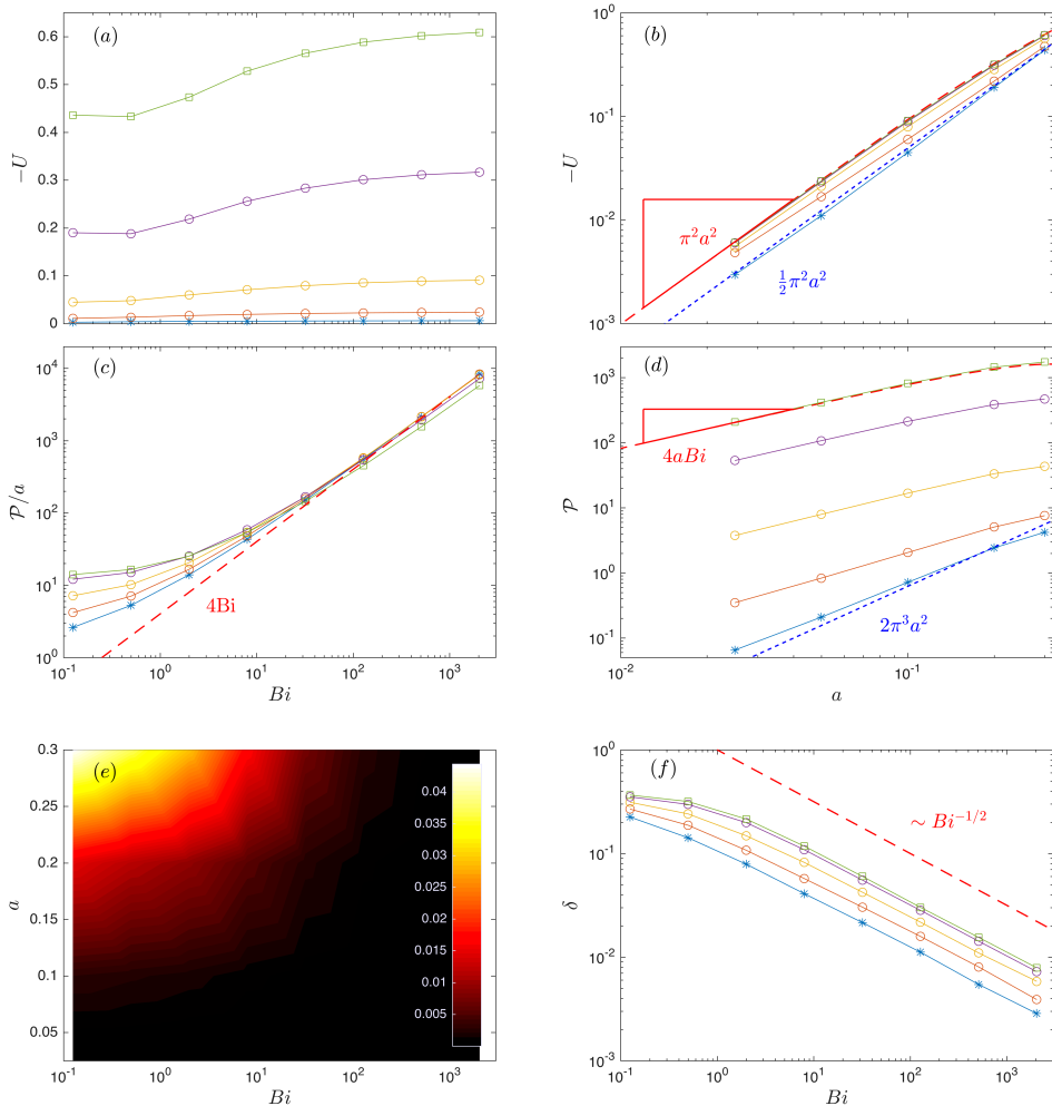
FIGURE 10. Data for longitudinal wave motion, for (a,c,f) different fixed amplitudes a = 0.025 , a = 0.05 , a = 0.1 , a = 0.2 and a = 0.3 , and for (b,d) different fixed Bingham numbers \text{Bi} = 1/8 , \text{Bi} = 2 , \text{Bi} = 32 , \text{Bi} = 512 and \text{Bi} = 2048 . For each plot, the series with the lowest (highest) value of the parameter ( a or \text{Bi} ) is marked with stars (squares) for clarity. (a, b) Swimming speed -U ; (c) scaled power consumption \mathcal{P}/a and (d) unscaled power consumption \mathcal{P} ; (e) a density plot of the efficiency \mathcal{E} = U^2/\mathcal{P} in (\text{Bi}, a) space; and (f) the thickness \delta of the yielded boundary layer above the sheet at x = 0 . Short-dashed (blue) lines lines show the theoretical predictions of §4.2 for a \ll 1 and \text{Bi} \ll 1 . The long-dashed (red) lines show the \text{Bi} \gg 1 predictions in (4.14) and (4.15) (with \text{Bi} = 2048 in (d)); the triangles indicate the limits for a \ll 1 .
