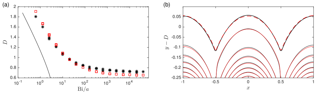
FIGURE 11. (a) Mean distance D from y = 0 to the upper yield surface, across a range of values of a and \text{Bi} for longitudinal waveforms (black stars), and compared with the same data for transverse waveforms from figure 6 (red squares). The solid line again shows D = y_B from (3.3). (b) The upper yield surface for longitudinal waveforms (black solid) translated by its mean distance D , compared with the same data for transverse waveforms (red dashed), shifted horizontally by 1/2 , for \text{Bi} = 1/8 and a = 0.025 . A few (equally spaced) streamlines in the laboratory frame are also shown for the longitudinal (black) and transverse (red) waves.
