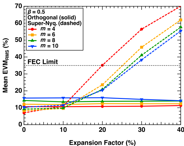
Fig. 6. Mean \text{EVM}_{\text{RMS}} dependence on the expansion factor ( \beta = 0.5 )
