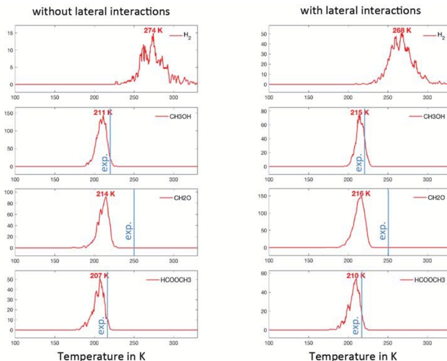
Figure 4. TPO spectra of methanol on Au(111) for scenario #1. The temperature ramp is 10 K/s. The initial coverage in \text{CH}_3\text{O} is 0.1 ML. The blue line corresponds to the approximate position of the experimental peak.
