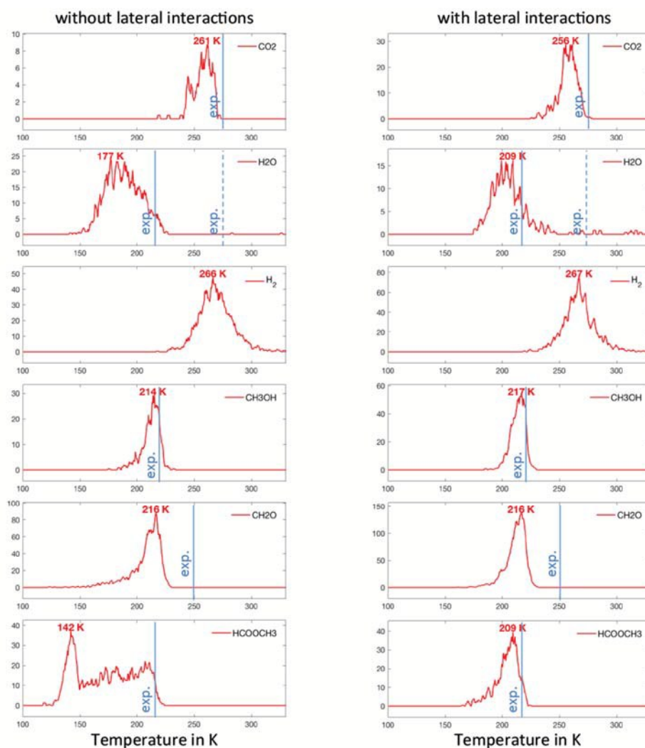
Figure 6. TPO spectra of methanol on Au(111) for scenario #3. Temperature ramp is 10 K/s. The initial coverages are: 0.1 ML of \text{CH}_3\text{O} and 0.02 ML in O.
