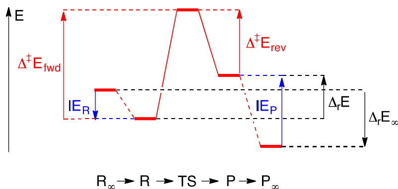
Figure 2. Energy diagram of the elementary process going from the reactant state R to the product state P via the transition state (TS). The state of infinitely separation of the reactants ( R_\infty ) and the products ( P_\infty ) are also indicated. In this example, there are attractive interactions between the reactant molecules and repulsive interactions between the products.
