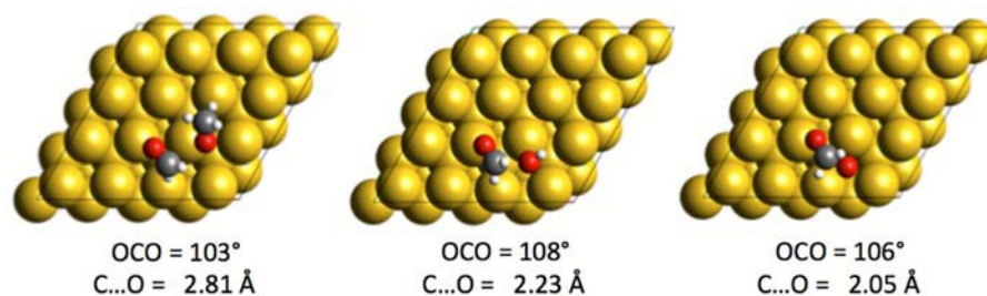
Figure 3. Structures of the three transition states associated with the A N 2 of O, OH and CH 3 O onto CH 2 O.
