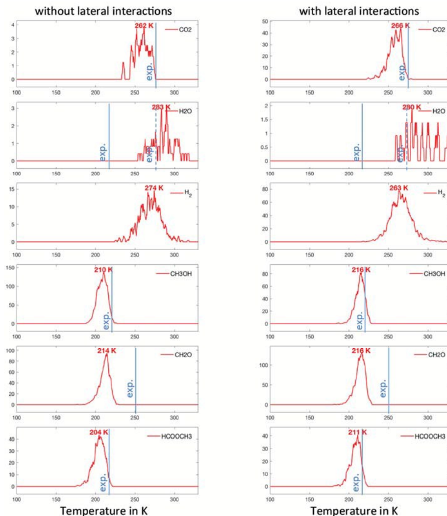
Figure 5. TPO spectra of methanol on Au(111) for scenario #2. Temperature ramp is 10 K/s. The initial coverages are: 0.1 ML of \text{CH}_3\text{O} and 0.02 ML in O.
