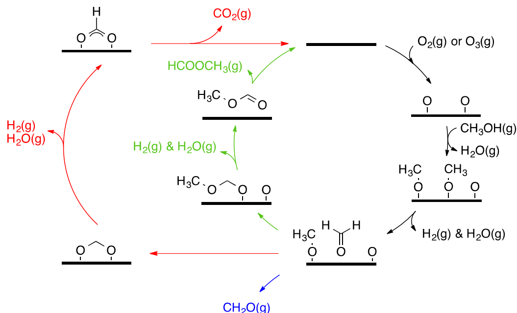
Figure 1. General mechanism for methanol oxidation over gold (represented as a thick horizontal line). The green arrows highlight the coupling while the red ones the over-oxidation route.
