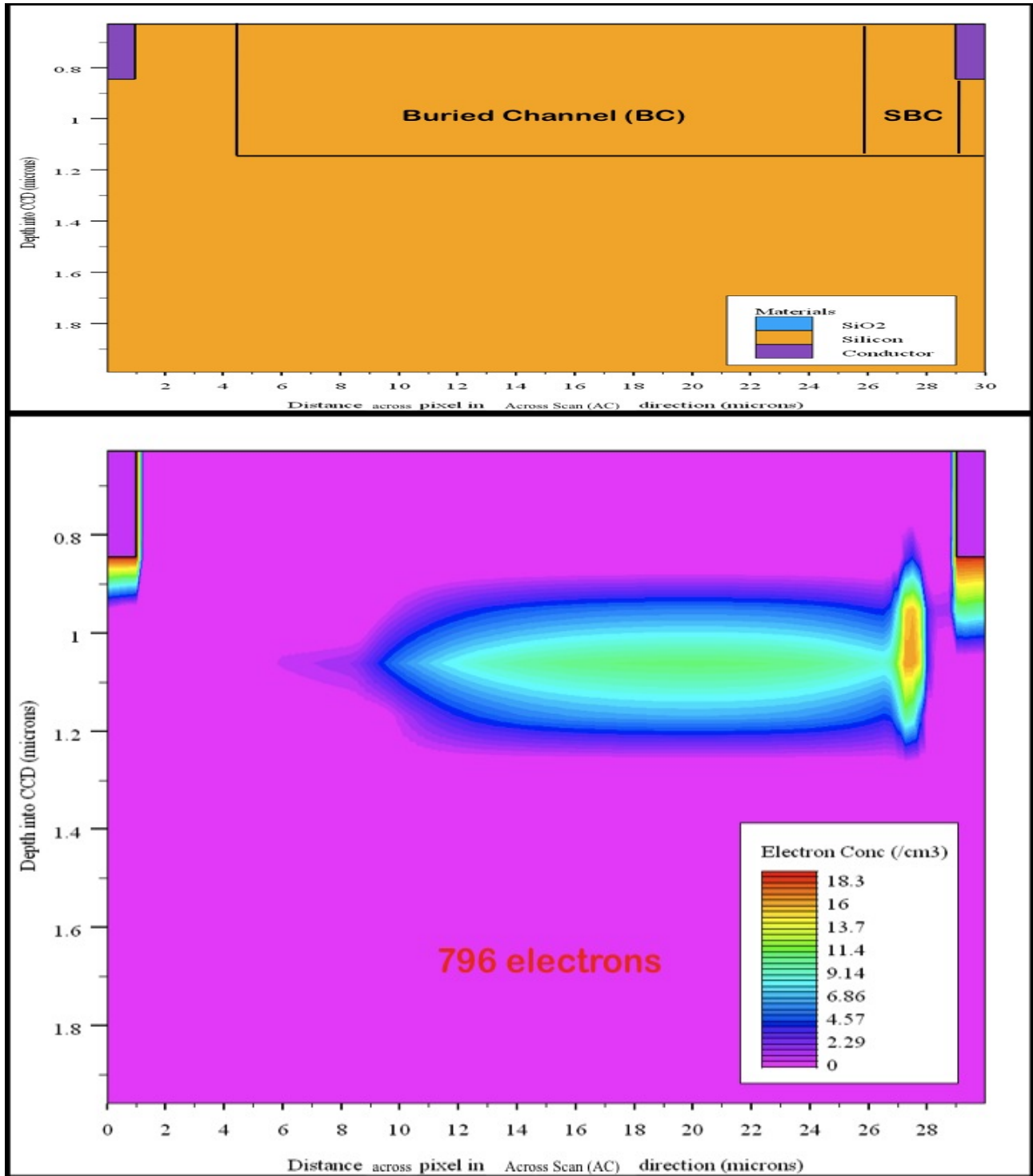
Fig. 4. Top : Plot shows the positions of the BC, SBC with nominal doping width of 3 \mu\text{m} and ABD (labeled as Conductor, shield doping not shown) as a function of CCD depth and distance across the pixel (perpendicular to the charge transfer direction). Bottom : Plot of electron concentration contours ( \text{dex}/\text{cm}^3 ) in a 1 \mu\text{m} thick cross-section through the centre of the AF pixel model in the charge transfer direction (and so approximately through the centre of the charge packet) overlying the top plot but simulated with SBC doping width of 2 \mu\text{m} . The BC contains less than one electron. Plots generated using the Silvaco plotting software TonyPlot.
