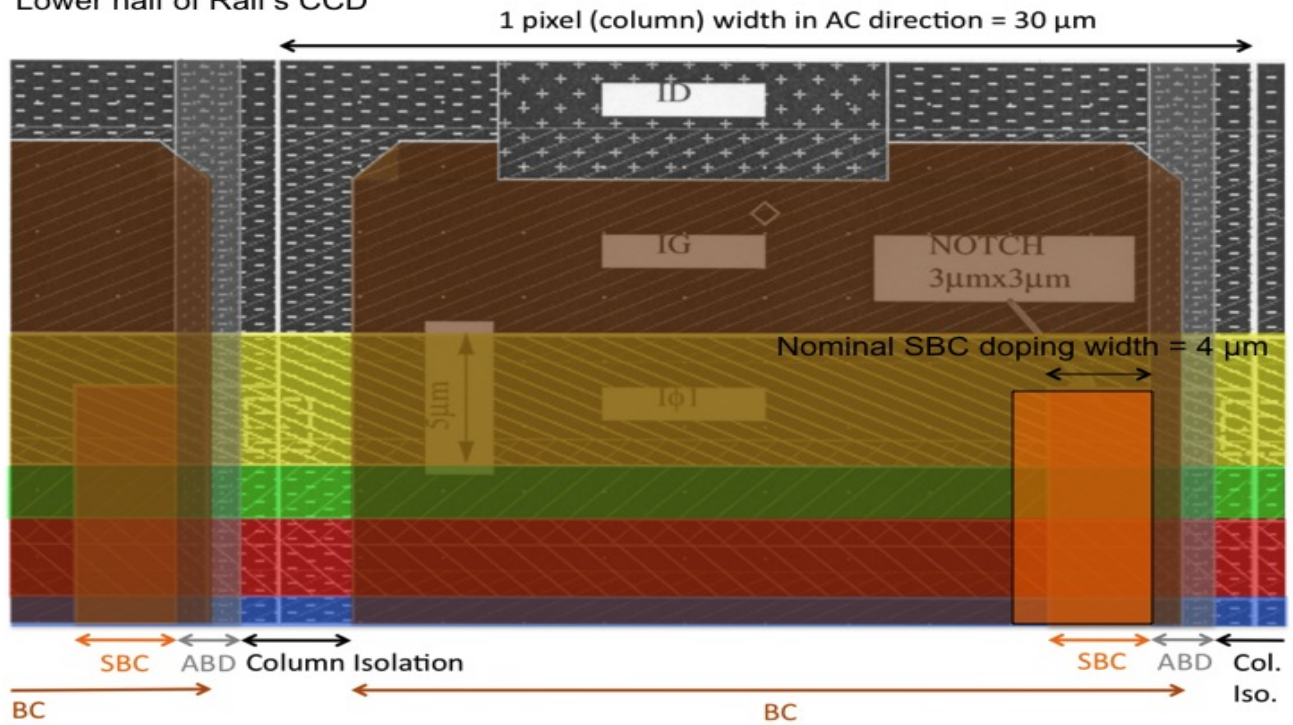
Lower half of Ralf's CCD
