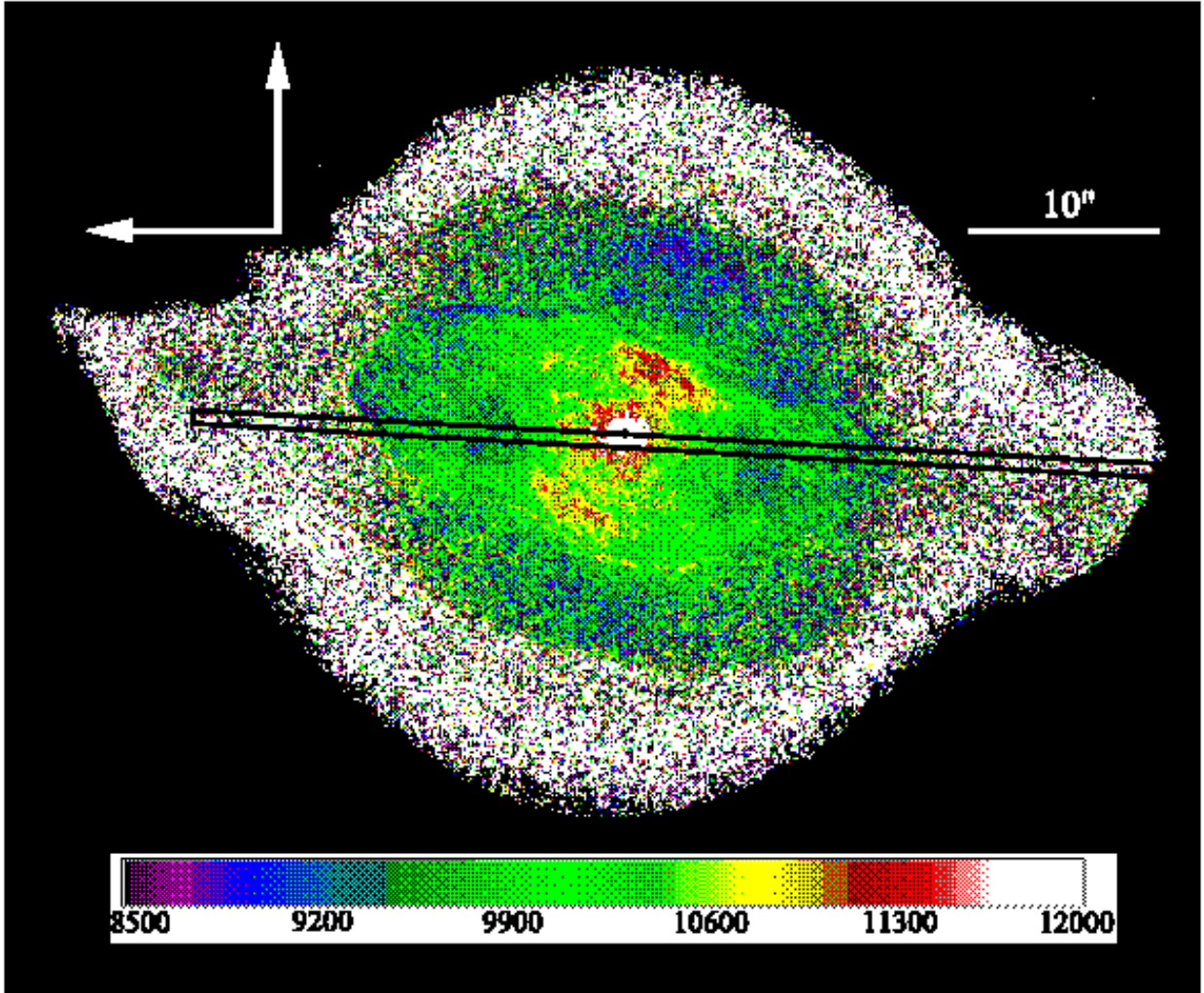
Fig. 2.— This is a pixel-by-pixel map of the electron temperature T_e (colour-bar scale) as determined from the ratio of extinction corrected fluxes of [O III] (4364 Å)/(5008 Å). The STIS long-slit (52" × 0.5") is aligned and superimposed on the image. The area representing the 0.5"-wide slit is shown fully unobstructed. The circumscribed black boundary lines are not part of the STIS slit. N is up and E to the left.
