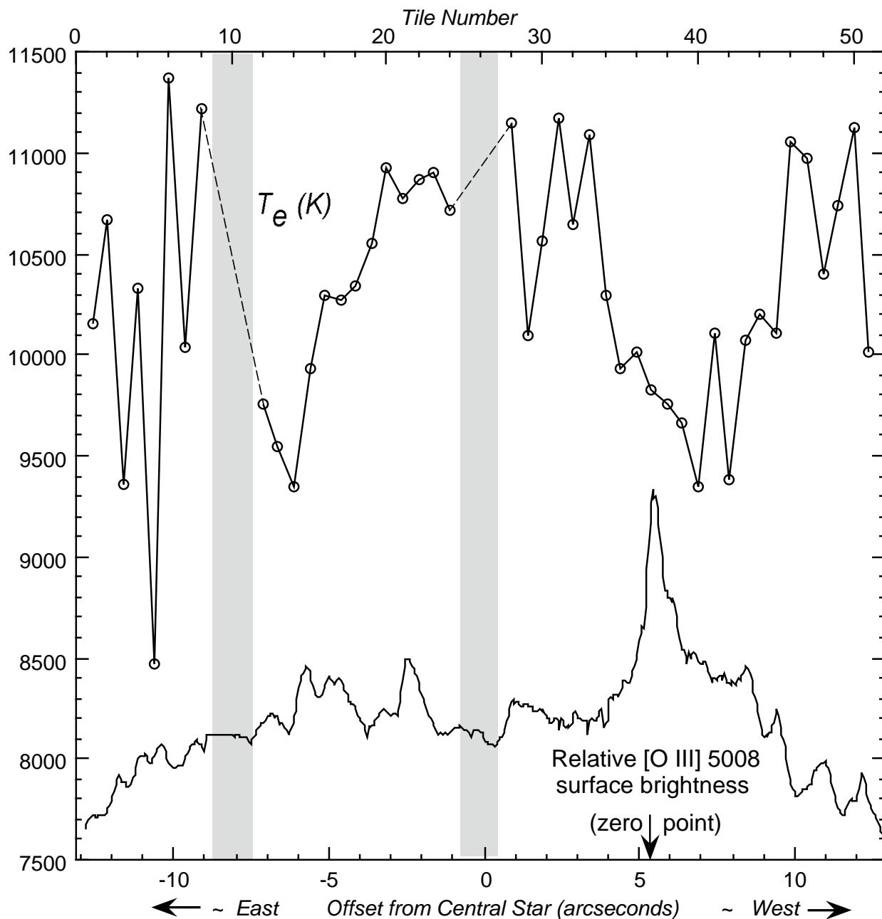
Fig. 1.— Plot of T_e determined from the [O III] 4364/5008 flux ratio vs. position along the STIS long-slit. The analysis is in terms of tiles that are 0.5'' square (matching the slit width). There are 45 tiles with reliable measurements that exclude the gray areas. The open circles represent the individual tiles plotted at their midpoint. The dashed straight lines are interpolations across the central star tiles (# 25–27) and across the east fiducial bar tiles (9–11). Tile # increases from \sim E to \sim W. The bottom curve shows the observed relative [O III] 5008 Å flux displayed unsmoothed at the pixel level.
